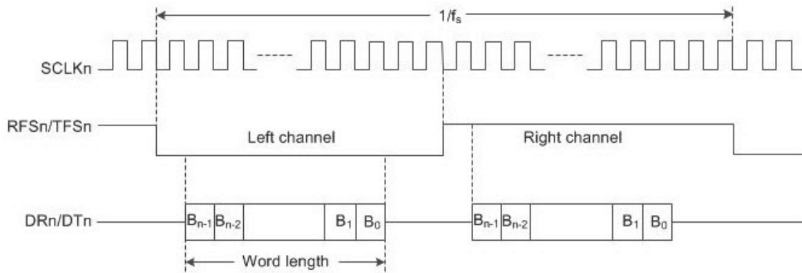
Figure 2-8. Timing for I 2 S Modes (both Master and Slave)
