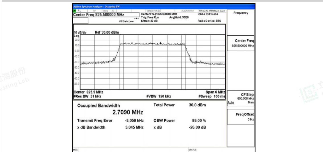
Band5-3MHz-QPSK-20525-15RB#0
