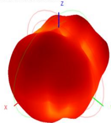
2450.0MHz H+V, Eff: 24.6%
