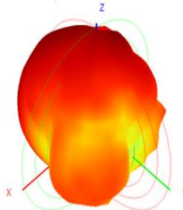
5850.0MHz H+V, Eff: 20.2%
