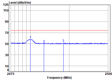
2.4G_SRD_1M_TX_CH_39_Horizontal-Peak
