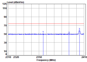
2.4G_SRD_2M_TX_CH_01_Vertical-Peak
