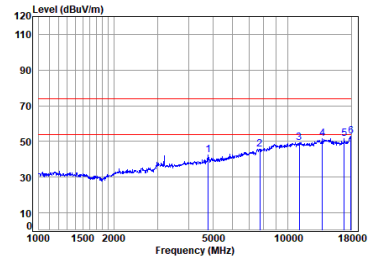
2.4G_SRD_TX_CH_00_Vertical
