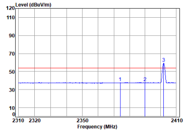
2.4G_SRD_1M_TX_CH_00_Horizontal-AVG
