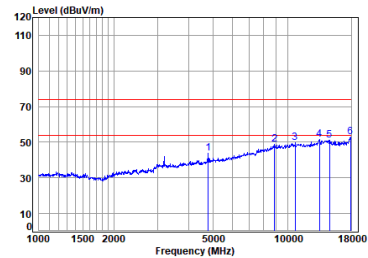
2.4G_SRD_TX_CH_19_Vertical
