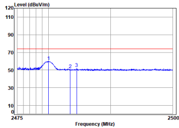
2.4G_SRD_1M_TX_CH_39_Vertical-Peak
