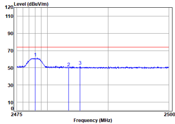
2.4G_SRD_2M_TX_CH_38_Horizontal-Peak
