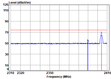
2.4G_SRD_2M_TX_CH_01_Horizontal-Peak
