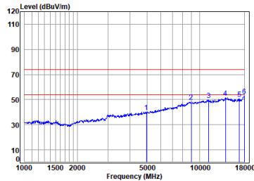
2.4G_SRD_TX_CH_00_Horizontal
