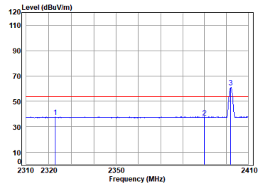
2.4G_SRD_1M_TX_CH_00_Vertical-AVG
