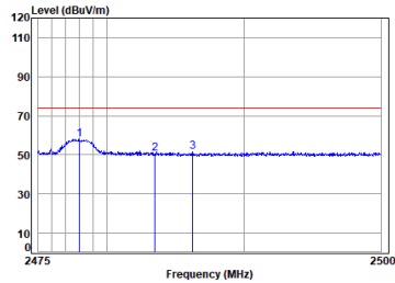
2.4G_SRD_2M_TX_CH_38_Vertical-Peak
