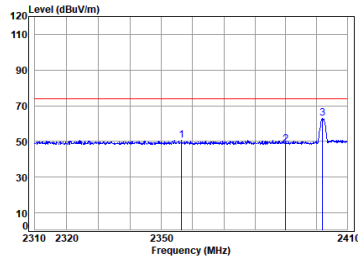
2.4G_SRD_1M_TX_CH_00_Horizontal-Peak
