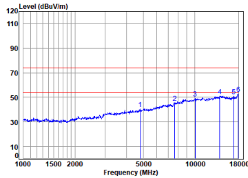
2.4G_SRD_2M_TX_CH_00_Horizontal
