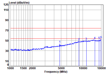
2.4G_SRD_2M_TX_CH_00_Vertical
