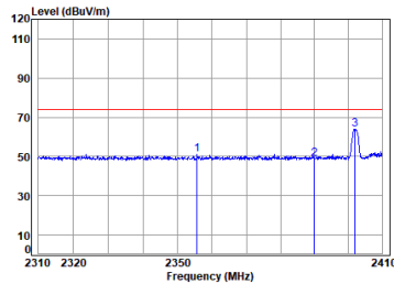
2.4G_SRD_1M_TX_CH_00_Vertical-Peak
