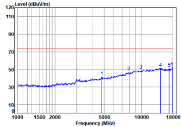
2.4G_SRD_2M_TX_CH_19_Vertical
