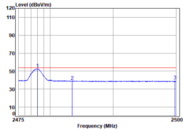
2.4G_SRD_1M_TX_CH_38_Vertical-AVG
