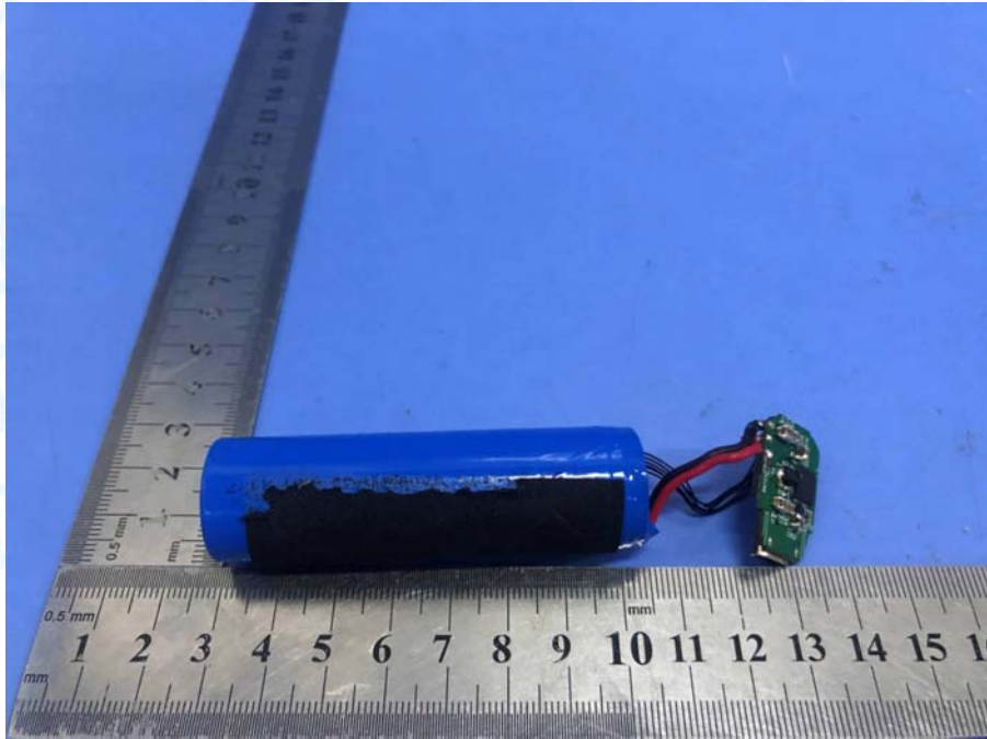
Photo 15 Appearance of PCB&Battery
