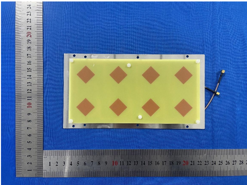
Photo 25: The product of DR5G17 Antenna view
