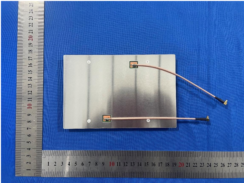
Photo 24: The product of DR5G15 Antenna view
