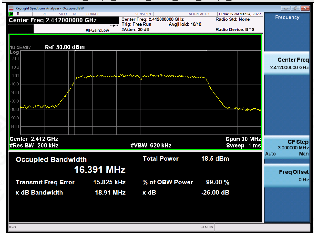
Test_Graph_802.11g_ANT1_2412_6Mbps_OBW
