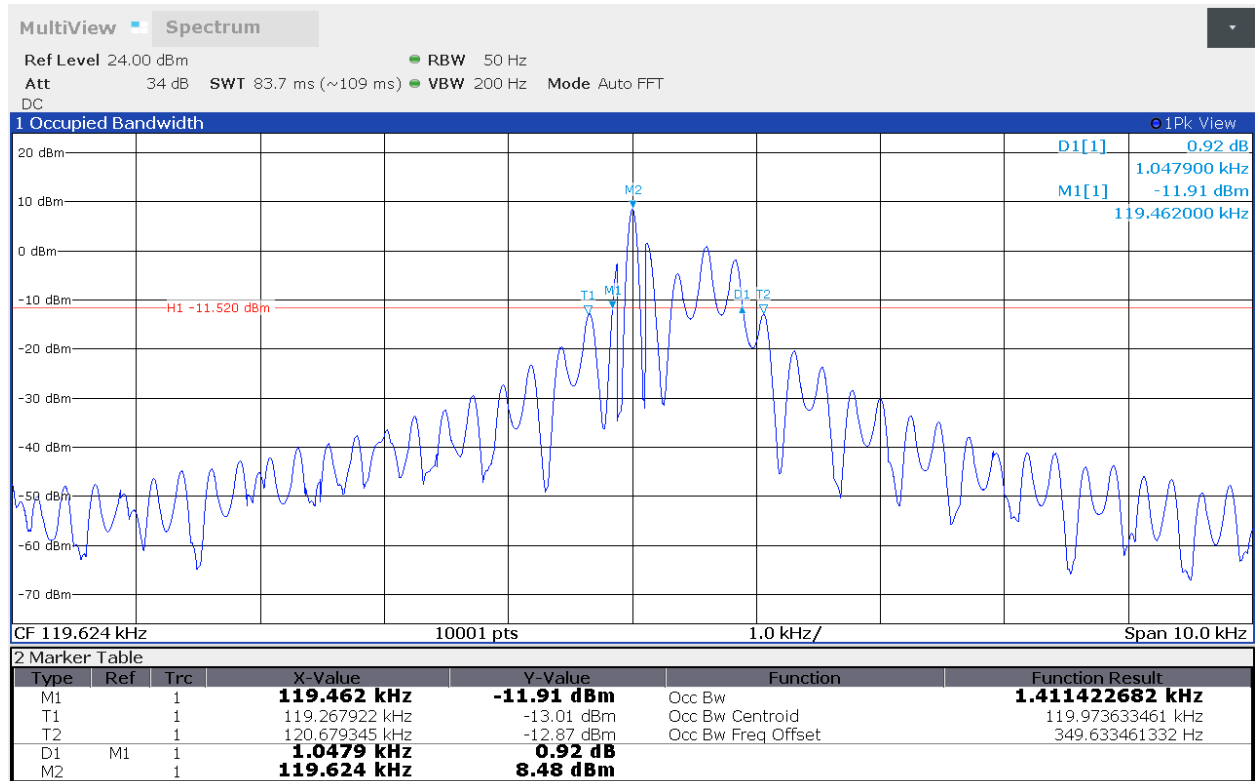
-20dB & 99% Channel Bandwidth Plot
