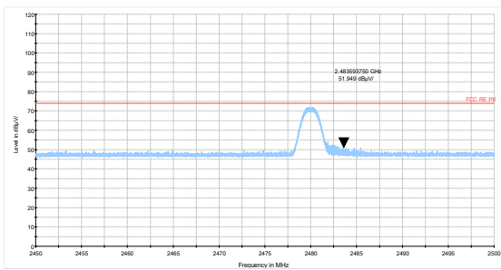
Bluetooth LE Channel 39 Peak
