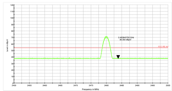
Bluetooth LE Channel 39 Average
