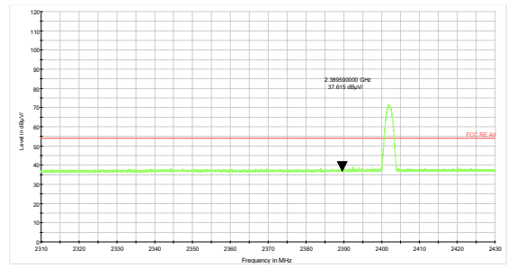
Bluetooth LE Channel 0 Average
