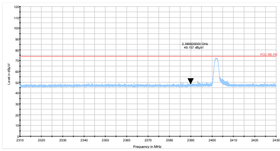
Bluetooth LE Channel 0 Peak
