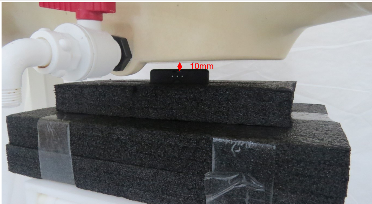
Picture 5: Top Side, the distance from handset to the bottom of the Phantom is 10mm
