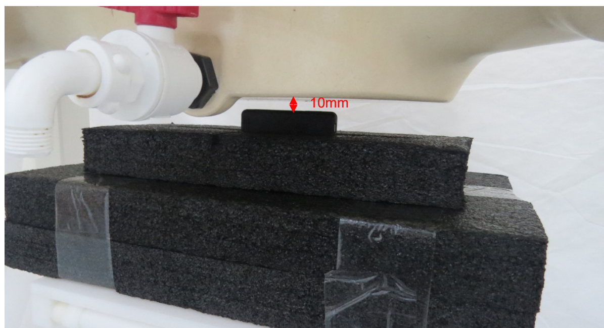
Picture 6: Bottom Edge, the distance from handset to the bottom of the Phantom is 10mm
