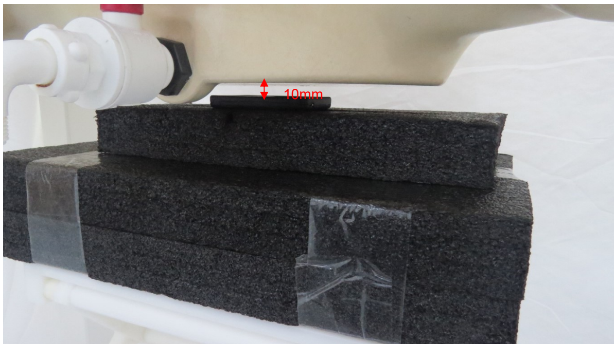
Picture 1: Back Side, the distance from handset to the bottom of the Phantom is 10mm
