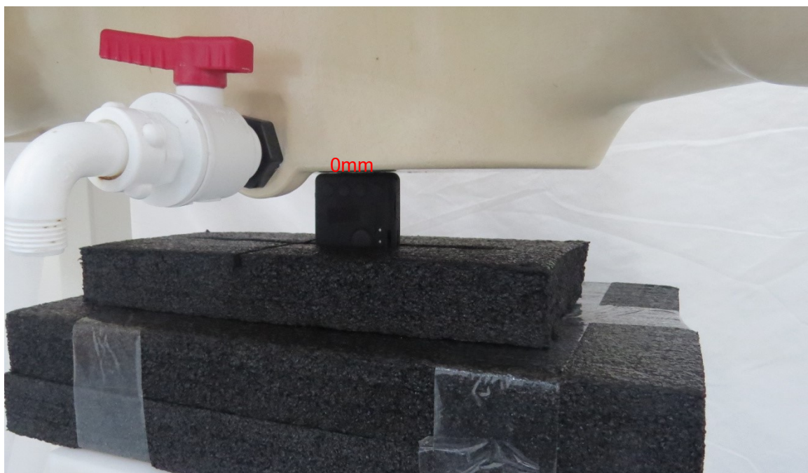
Picture 9: Left Side, the distance from handset to the bottom of the Phantom is 0mm
