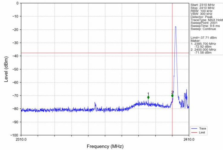
GFSK_DH5_LCH_2402MHz_Ant1_NTNV
