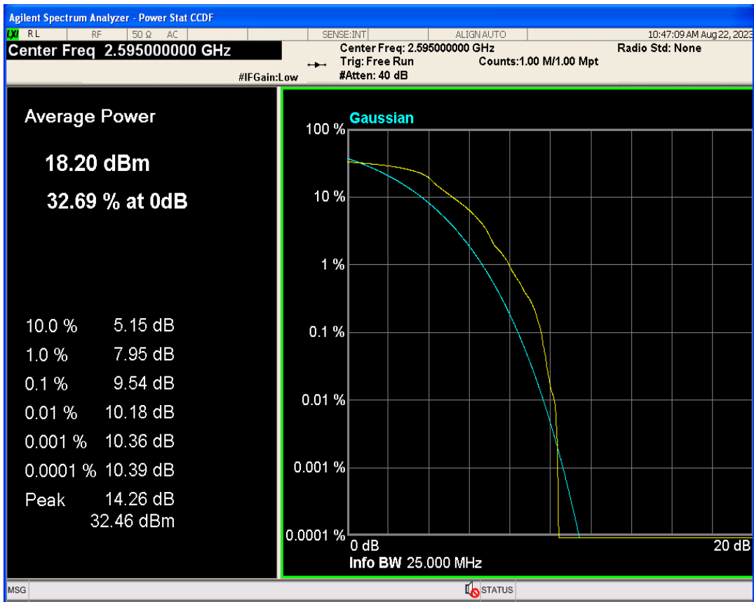
Band41a 16QAM BW=15MHz Channel=40640 RB Size=1 Position=#0
