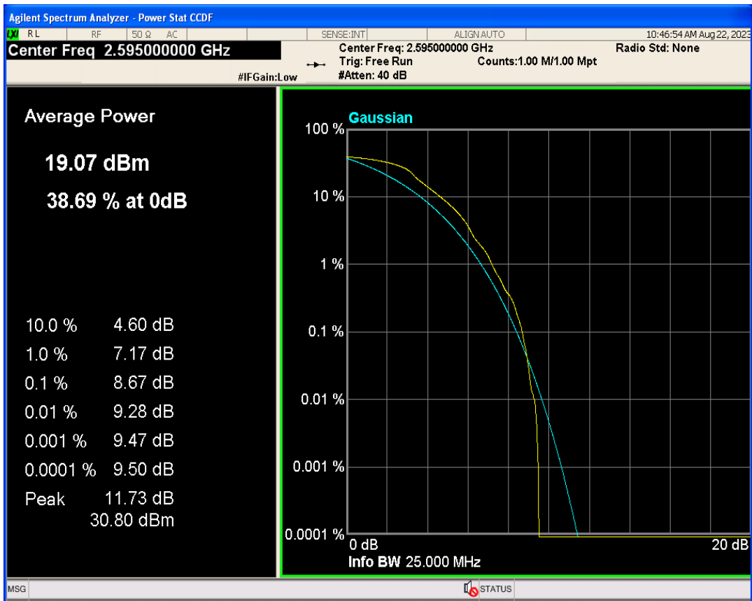
Band41a 16QAM BW=10MHz Channel=40640 RB Size=1 Position=#0
