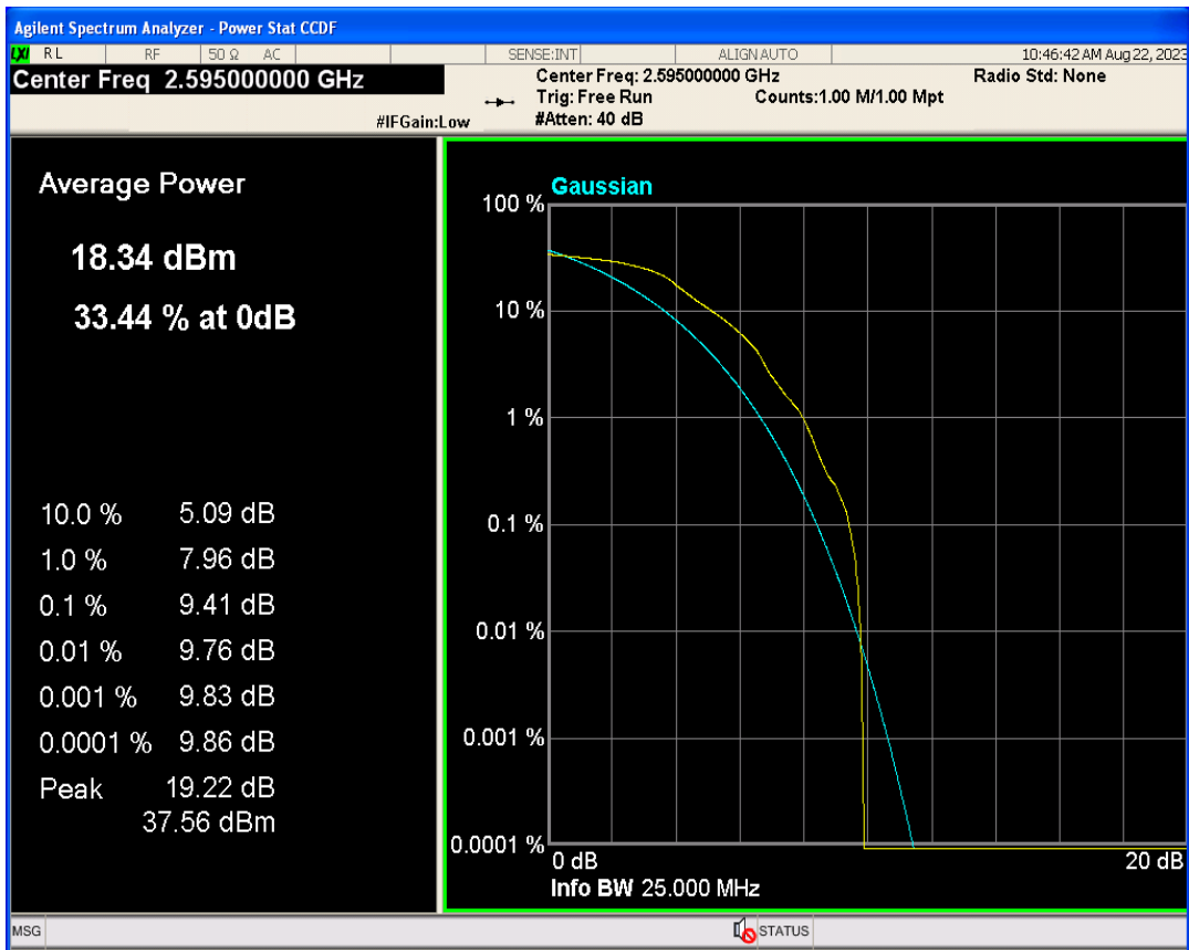
Band41a 16QAM BW=5MHz Channel=40640 RB Size=1 Position=#0
