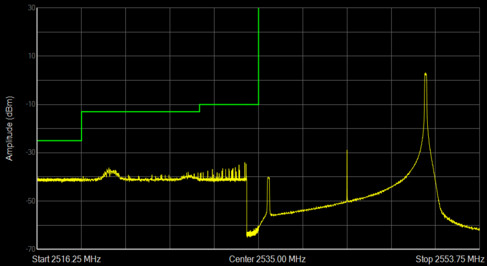
Band41a QPSK BW=15MHz Channel=40115 RB Size=1 Position=#Max
