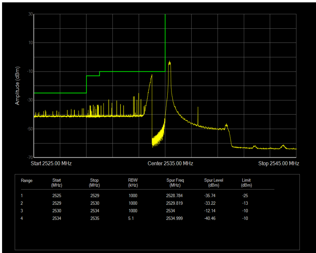
Band41a QPSK BW=5MHz Channel=40065 RB Size=1 Position=#Max
