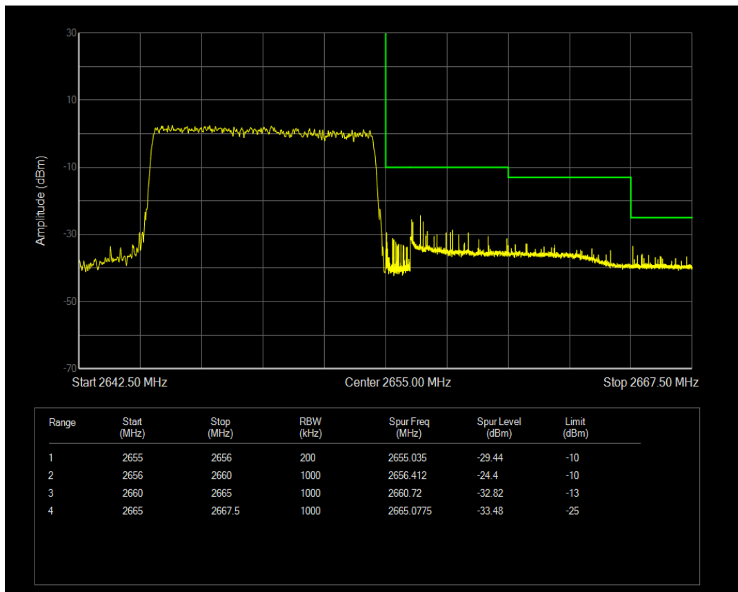
Band41a 16QAM BW=10MHz Channel=41190 RB Size=1 Position=#0
