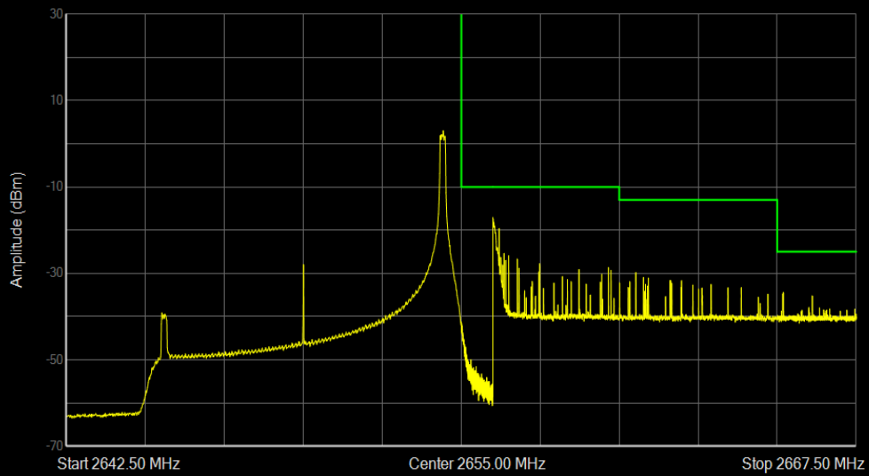
Band41a 16QAM BW=10MHz Channel=41190 RB Size=1 Position=#Max
