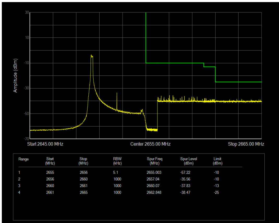
Band41a QPSK BW=5MHz Channel=41215 RB Size=1 Position=#Max
