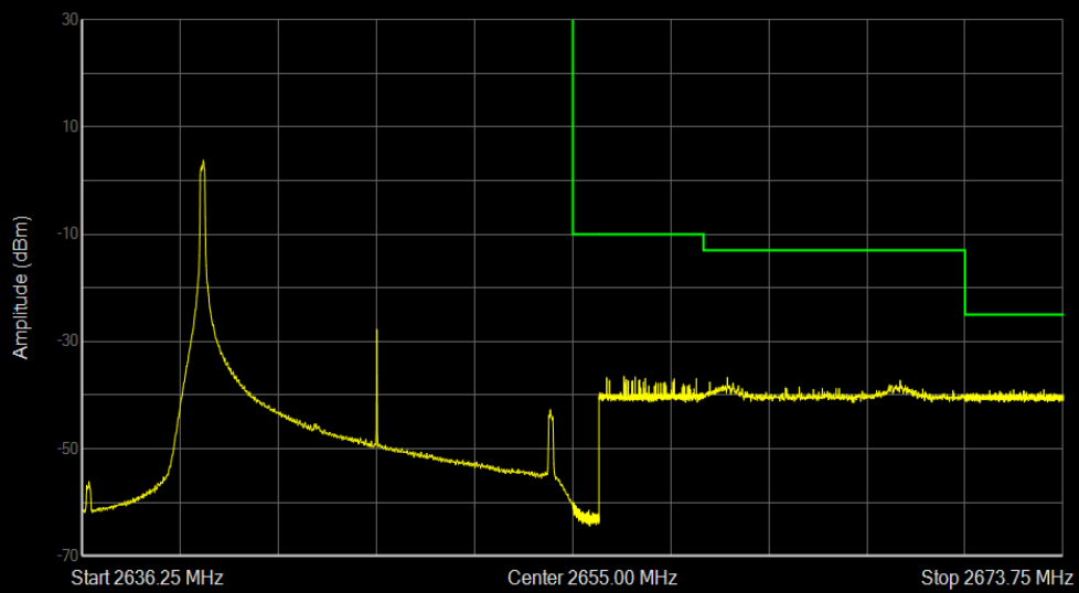
Band41a QPSK BW=15MHz Channel=41165 RB Size=1 Position=#0
