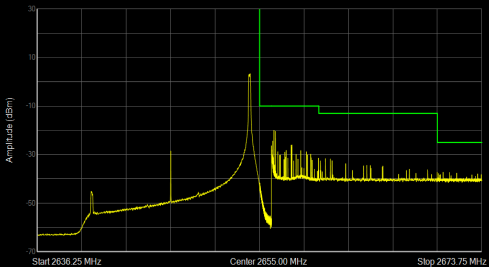
Band41a QPSK BW=15MHz Channel=41165 RB Size=1 Position=#Max
