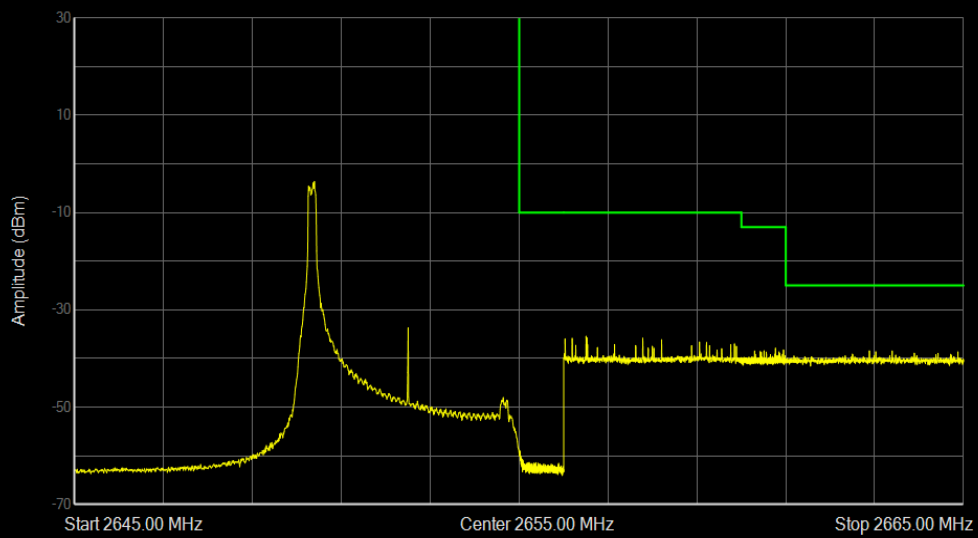
Band41a 16QAM BW=5MHz Channel=41215 RB Size=1 Position=#0
