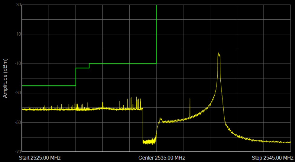
Band41a 16QAM BW=5MHz Channel=40065 RB Size=1 Position=#Max
