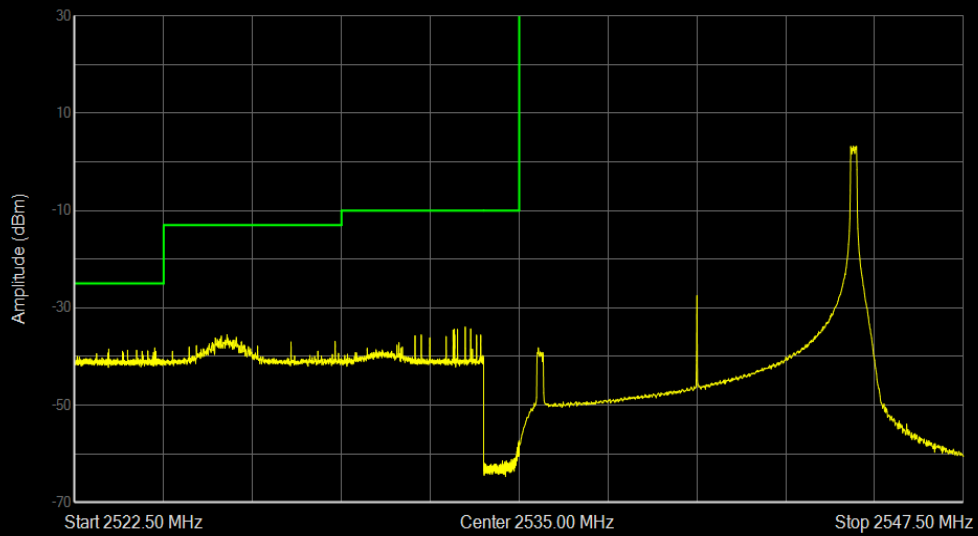
Band41a QPSK BW=10MHz Channel=40090 RB Size=1 Position=#Max
