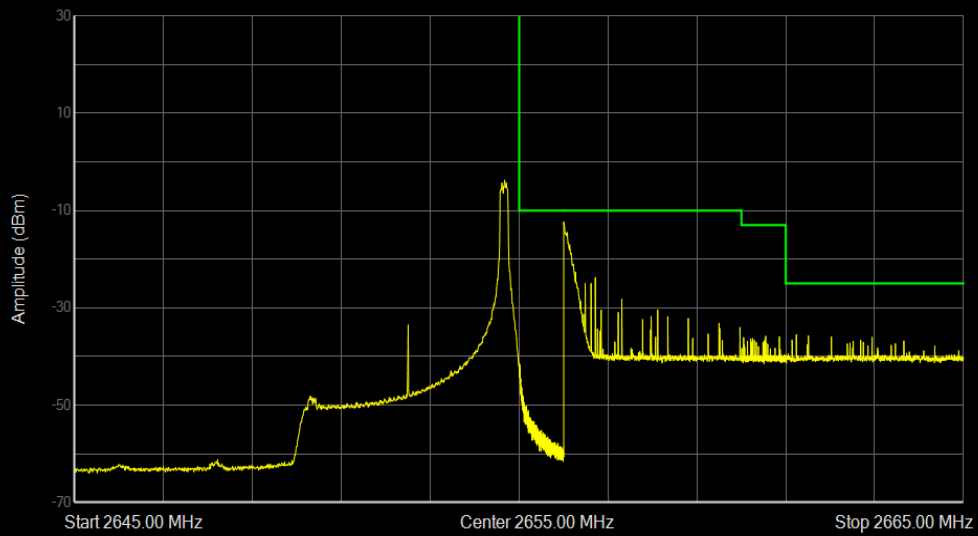
Band41a 16QAM BW=5MHz Channel=41215 RB Size=1 Position=#Max
