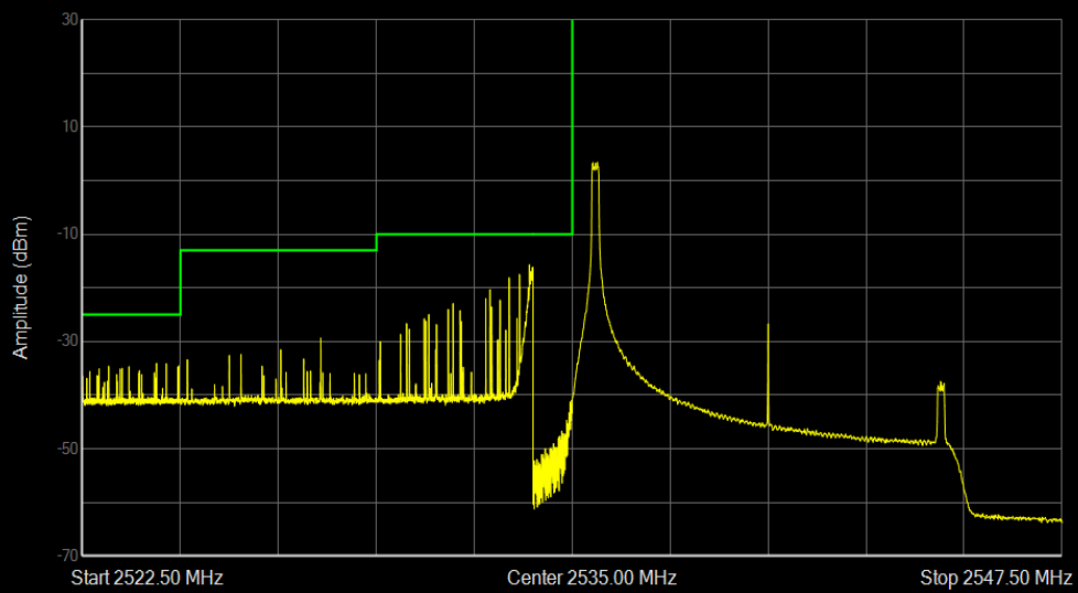
Band41a QPSK BW=10MHz Channel=40090 RB Size=1 Position=#0
