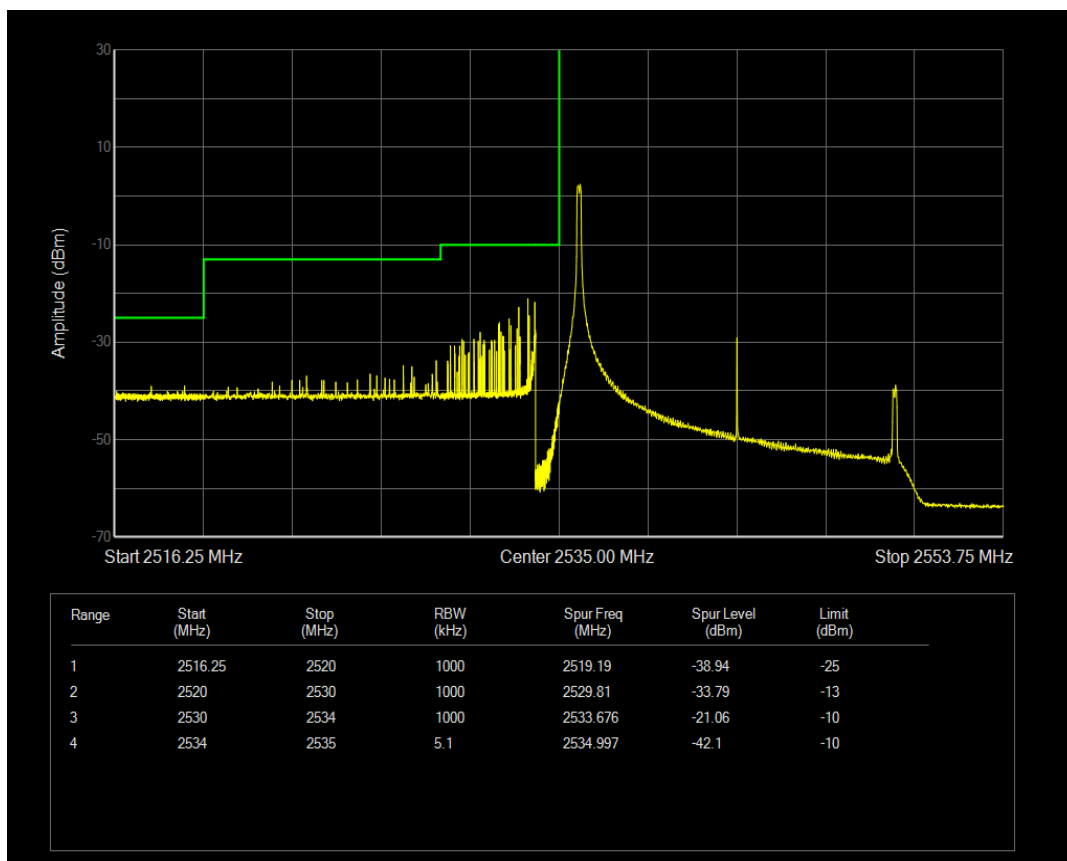
Band41a 16QAM BW=15MHz Channel=40115 RB Size=1 Position=#Max
