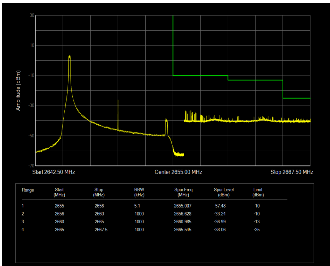
Band41a QPSK BW=10MHz Channel=41190 RB Size=1 Position=#Max
