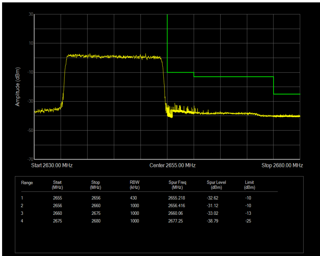
Band41a 16QAM BW=20MHz Channel=41140 RB Size=1 Position=#0
