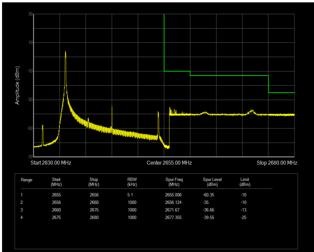
Band41a QPSK BW=20MHz Channel=41140 RB Size=1 Position=#Max
