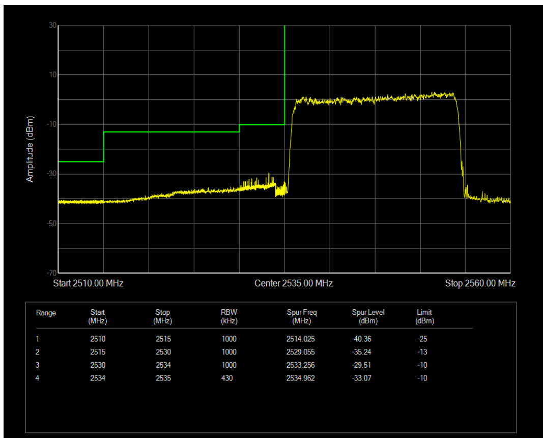
Band41a 16QAM BW=20MHz Channel=40140 RB Size=1 Position=#0
