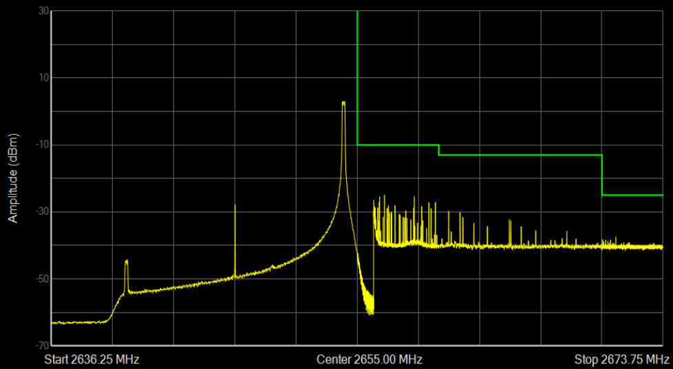
Band41a 16QAM BW=15MHz Channel=41165 RB Size=1 Position=#Max
