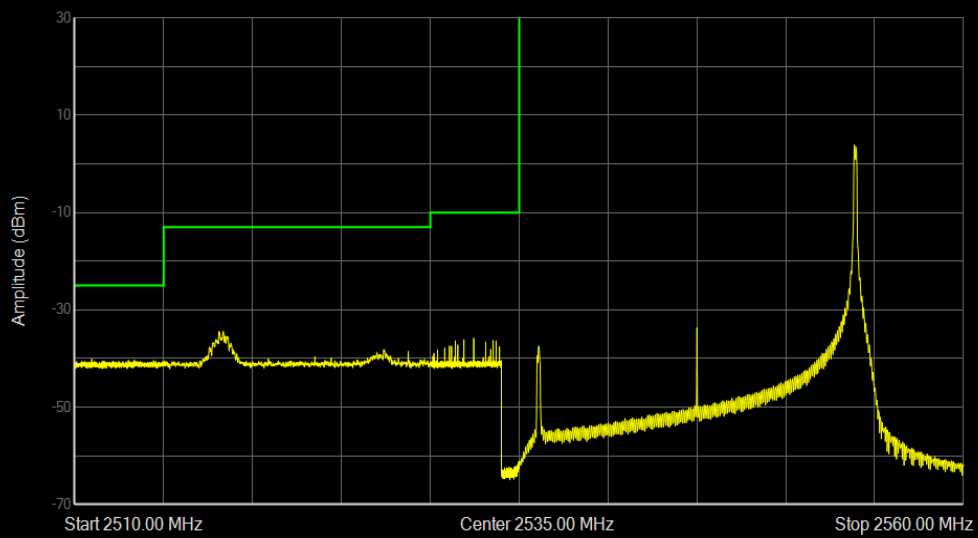
Band41a 16QAM BW=20MHz Channel=40140 RB Size=1 Position=#Max
