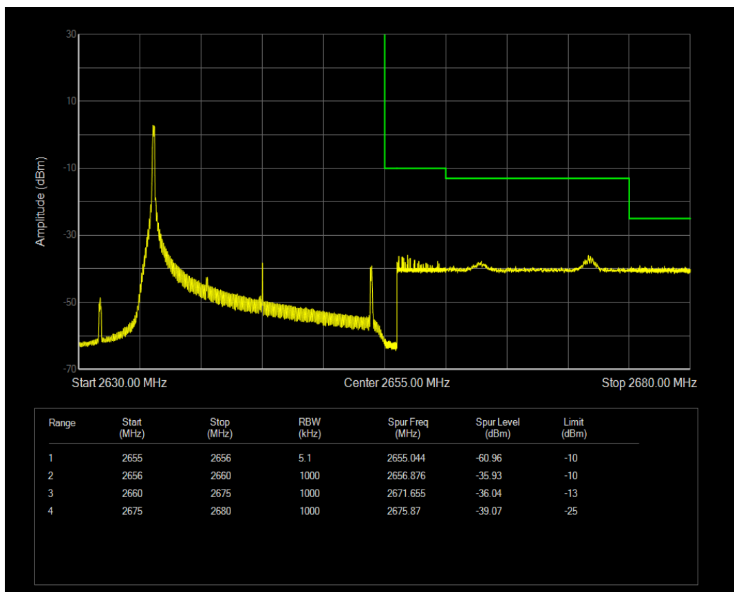
Band41a 16QAM BW=20MHz Channel=41140 RB Size=1 Position=#Max
