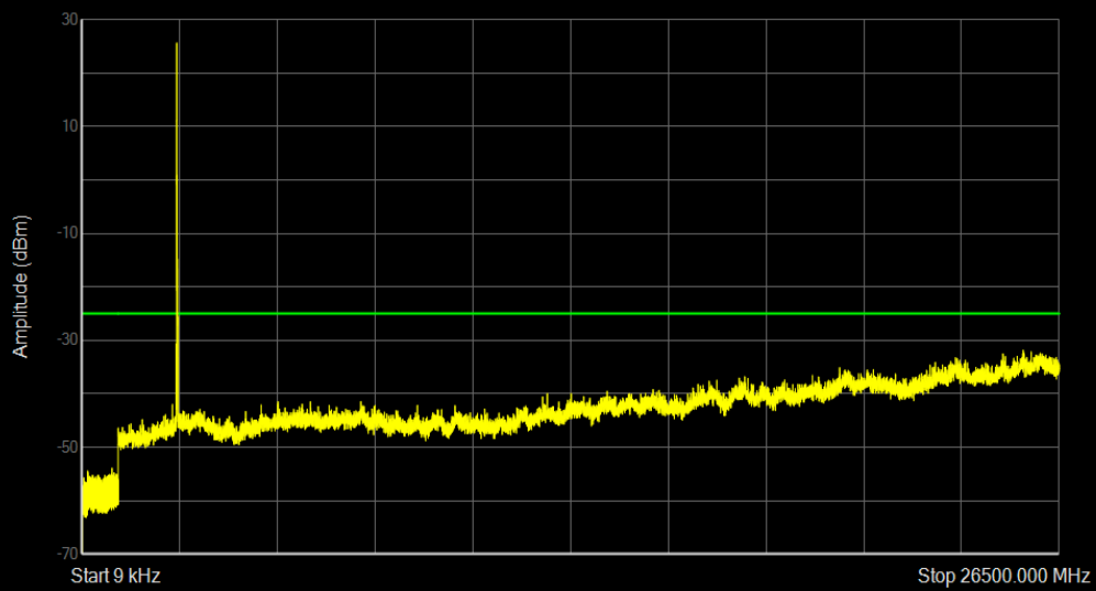
Band38 QPSK BW=15MHz Channel=38000 RB Size=1 Position=#0
