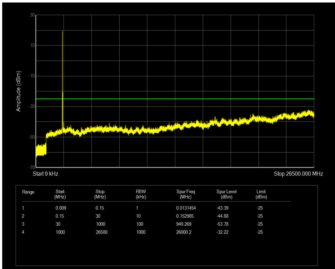
Band41a QPSK BW=10MHz Channel=40640 RB Size=1 Position=#0
