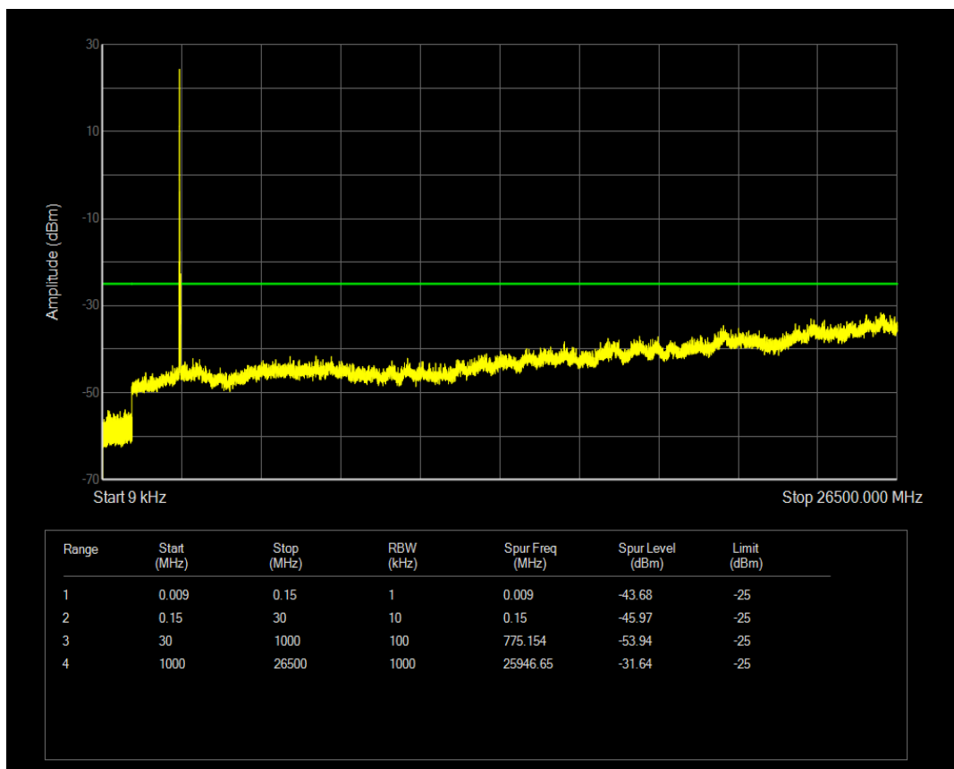
Band41a 16QAM BW=15MHz Channel=40640 RB Size=1 Position=#0
