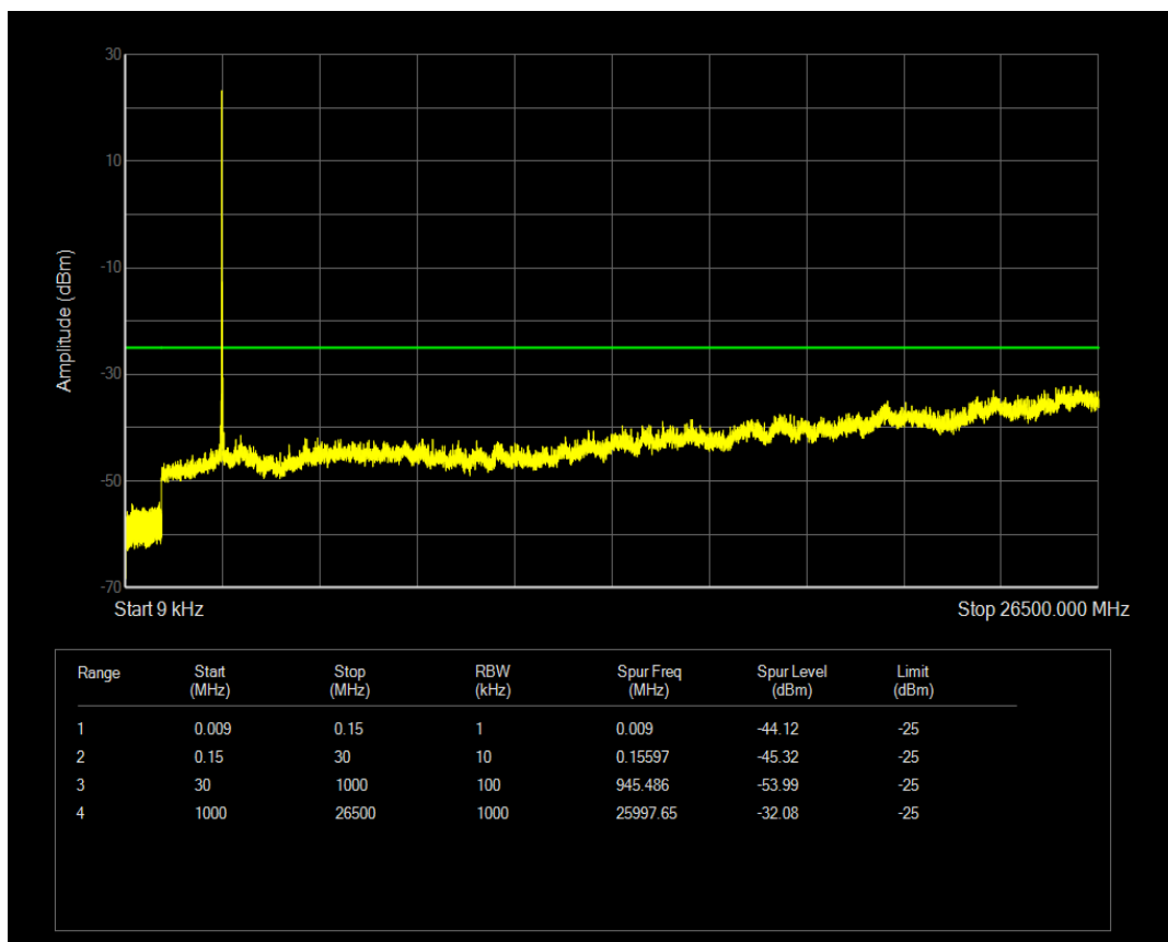
Band41a 16QAM BW=15MHz Channel=41165 RB Size=75 Position=#0
