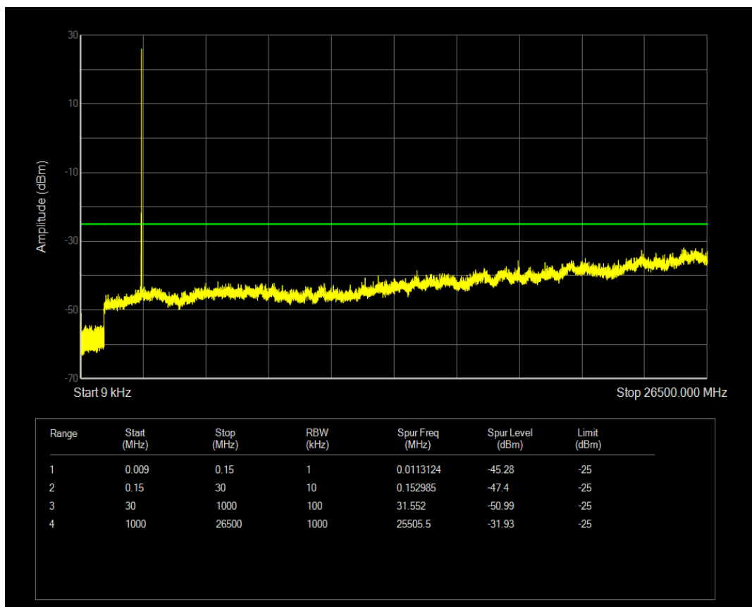
Band41a 16QAM BW=5MHz Channel=40640 RB Size=25 Position=#0
