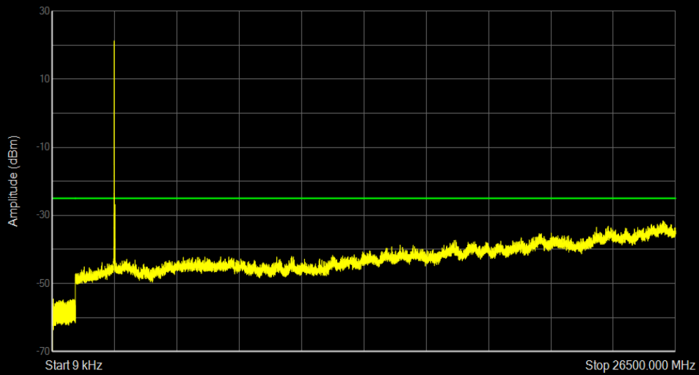
Band41a QPSK BW=5MHz Channel=41215 RB Size=25 Position=#0
