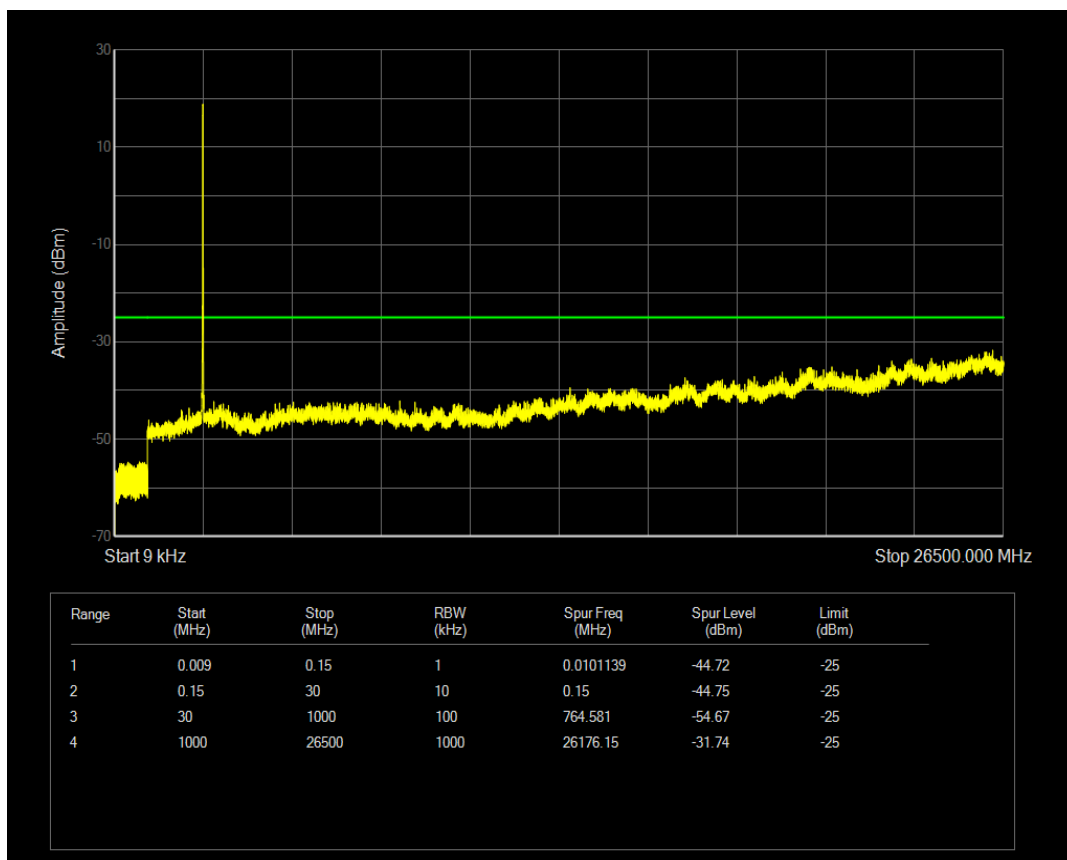
Band41a 16QAM BW=10MHz Channel=41190 RB Size=1 Position=#0
