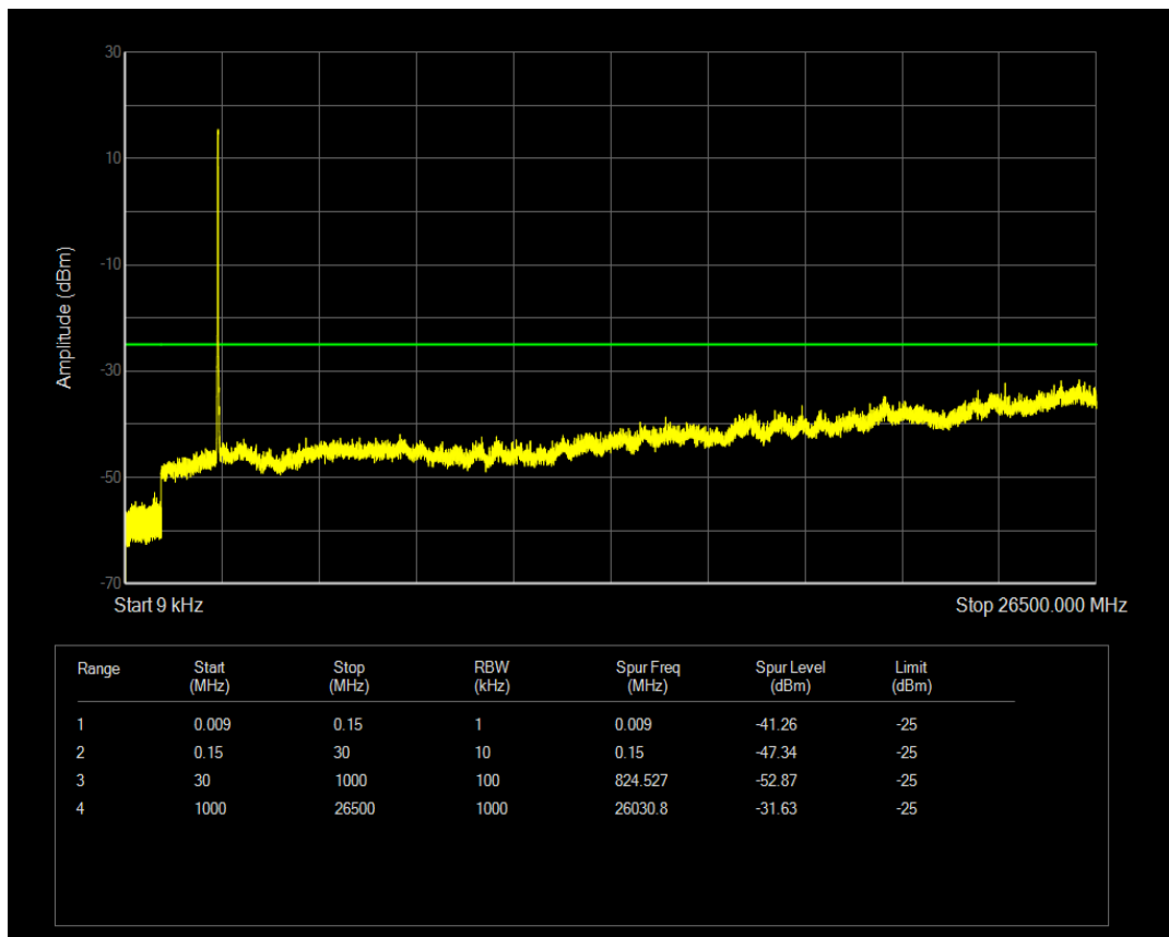
Band41a QPSK BW=20MHz Channel=40640 RB Size=1 Position=#0
