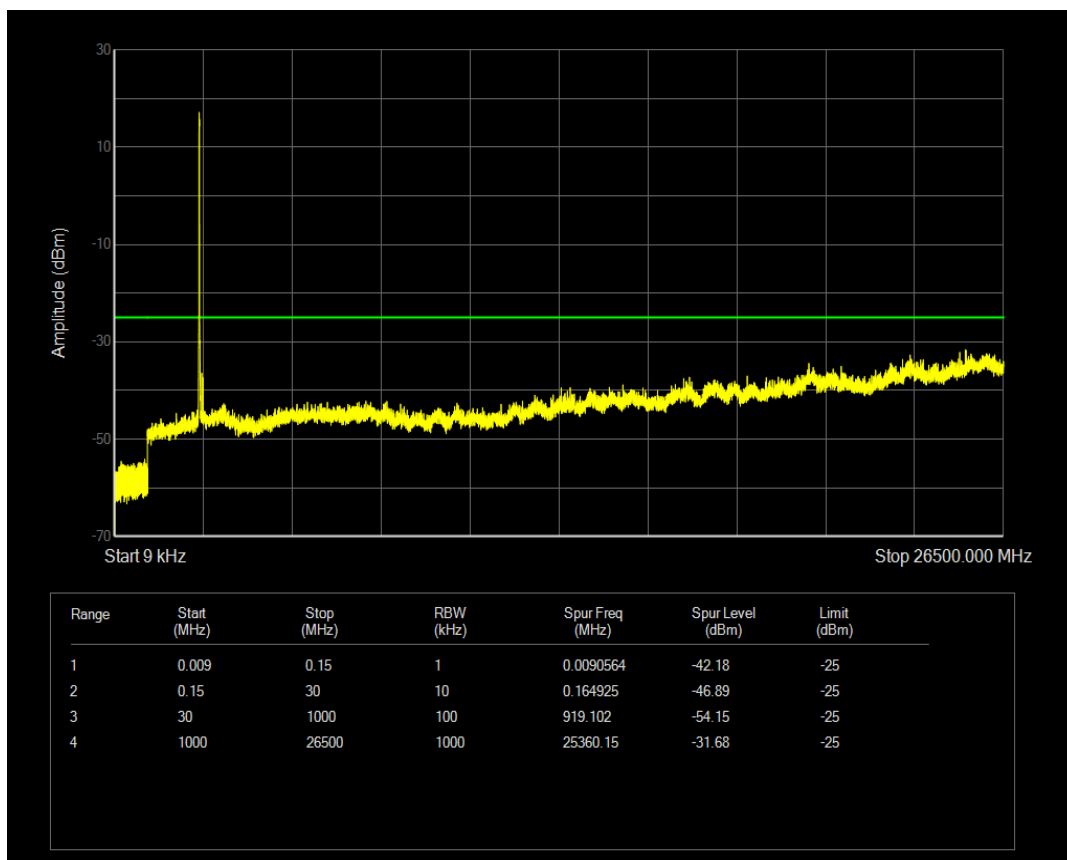
Band41a QPSK BW=15MHz Channel=40640 RB Size=1 Position=#0
