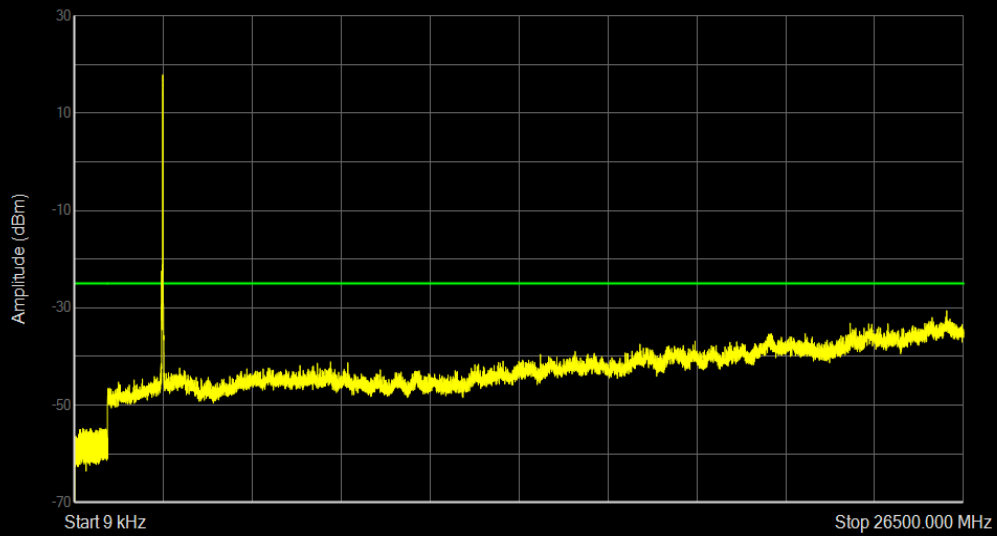
Band41a QPSK BW=15MHz Channel=41165 RB Size=75 Position=#0
