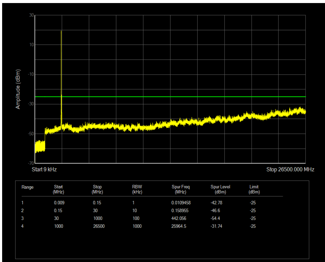
Band41a 16QAM BW=10MHz Channel=40640 RB Size=50 Position=#0
