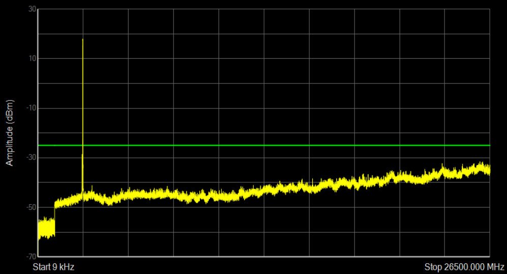
Band41a 16QAM BW=10MHz Channel=41190 RB Size=50 Position=#0
