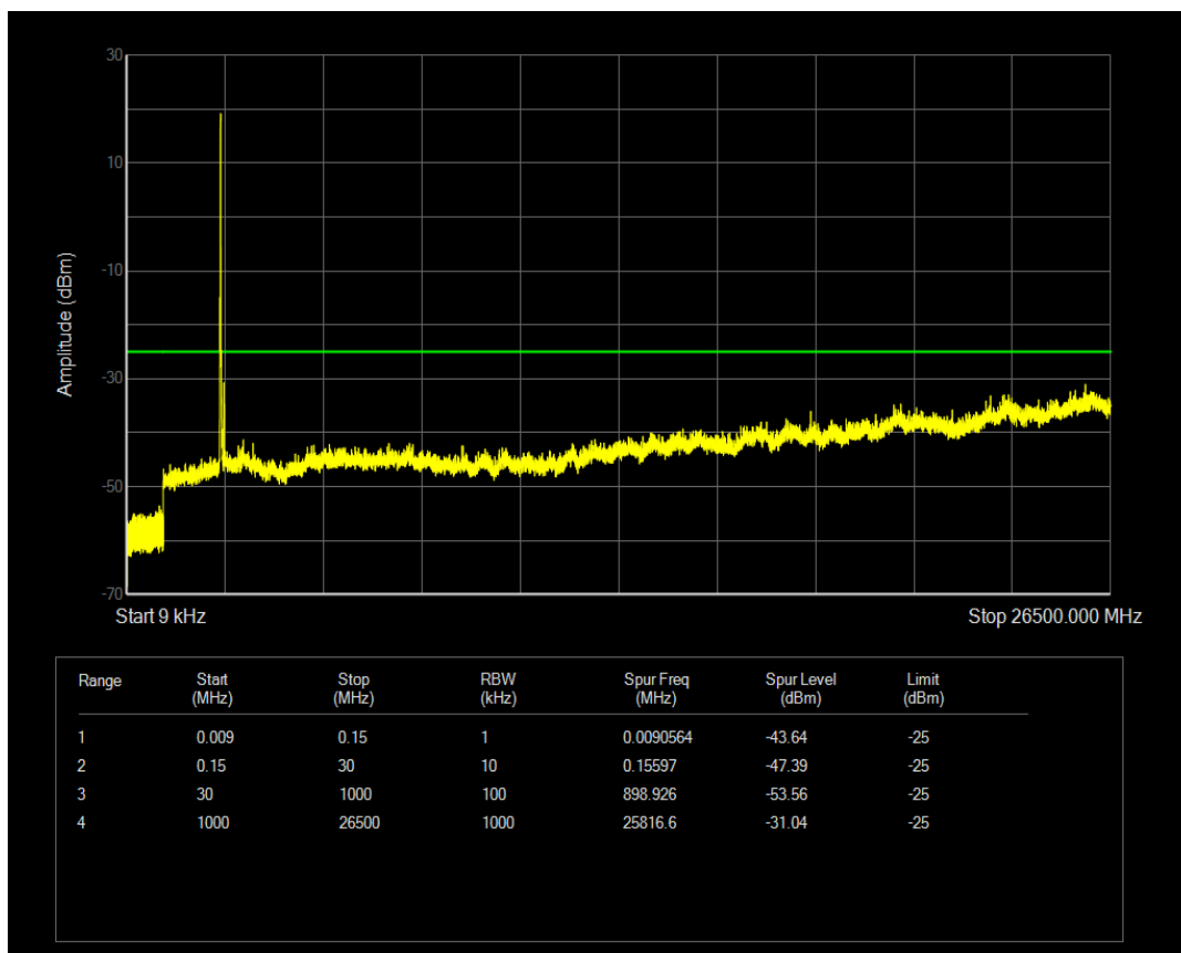
Band41a QPSK BW=15MHz Channel=40115 RB Size=1 Position=#0
