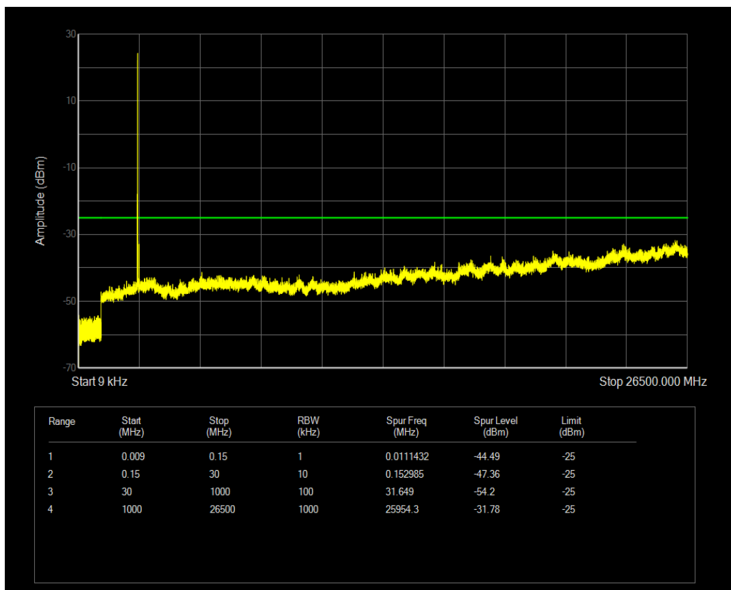
Band41a QPSK BW=5MHz Channel=40640 RB Size=25 Position=#0
