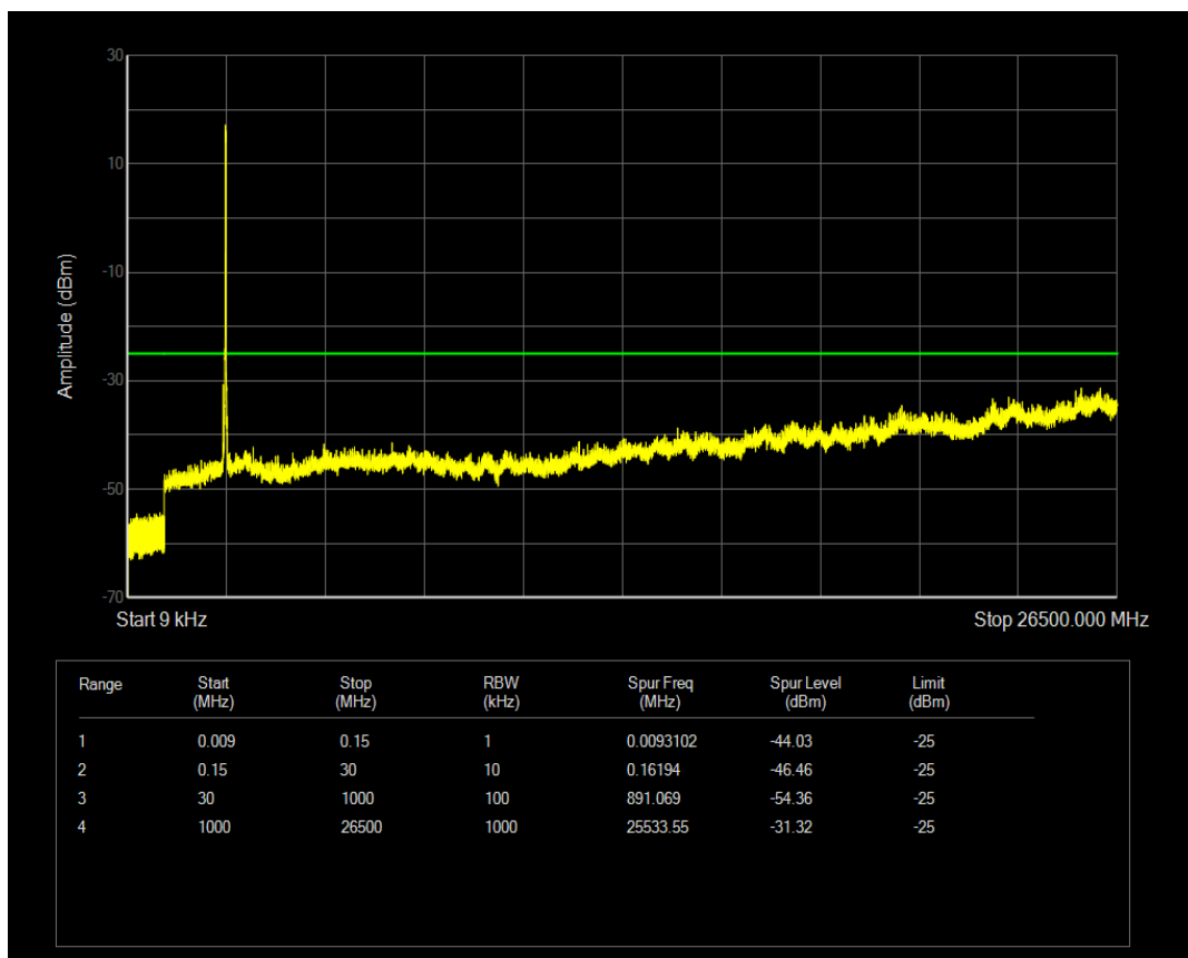
Band41a 16QAM BW=20MHz Channel=41140 RB Size=1 Position=#0
