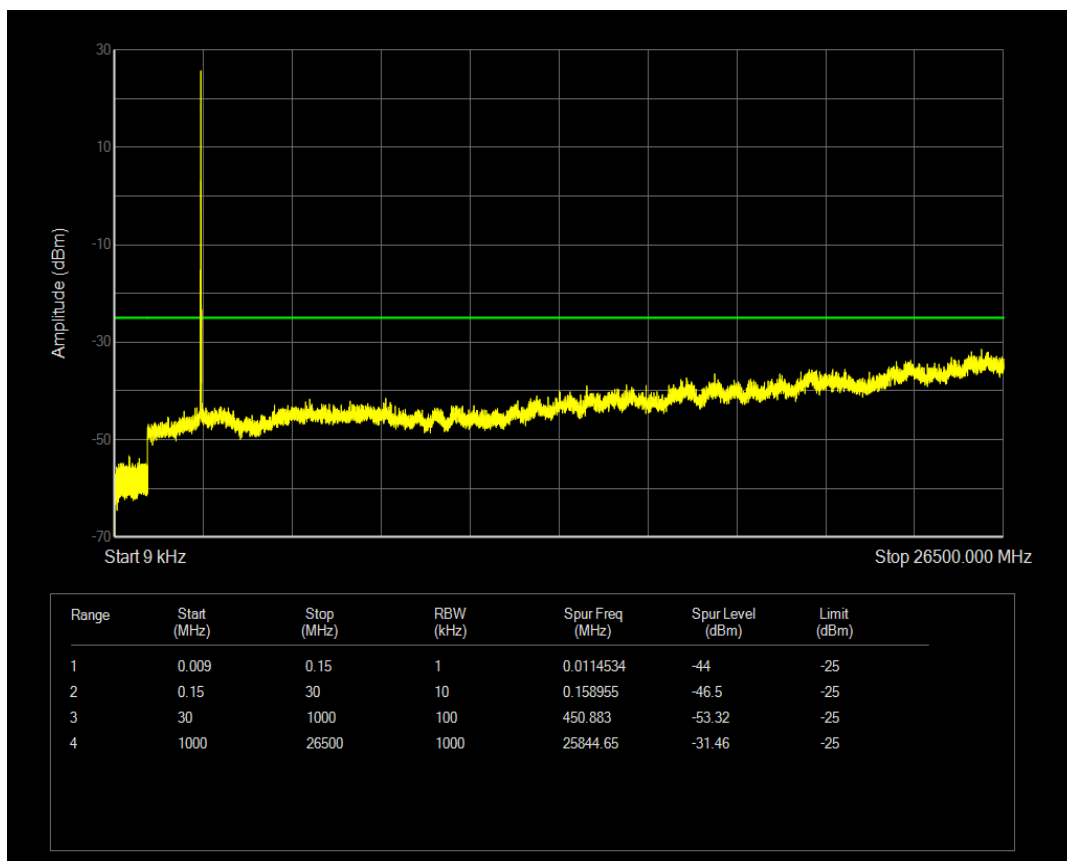
Band41a QPSK BW=10MHz Channel=40640 RB Size=50 Position=#0
