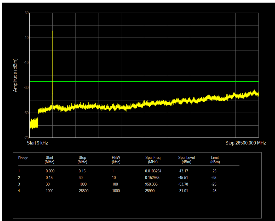
Band41a QPSK BW=20MHz Channel=40140 RB Size=1 Position=#0
