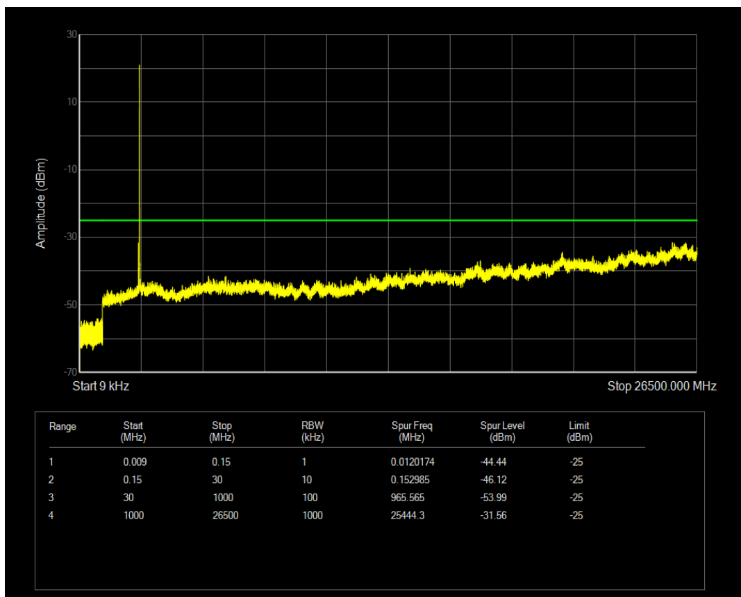
Band41a 16QAM BW=5MHz Channel=40640 RB Size=1 Position=#0
