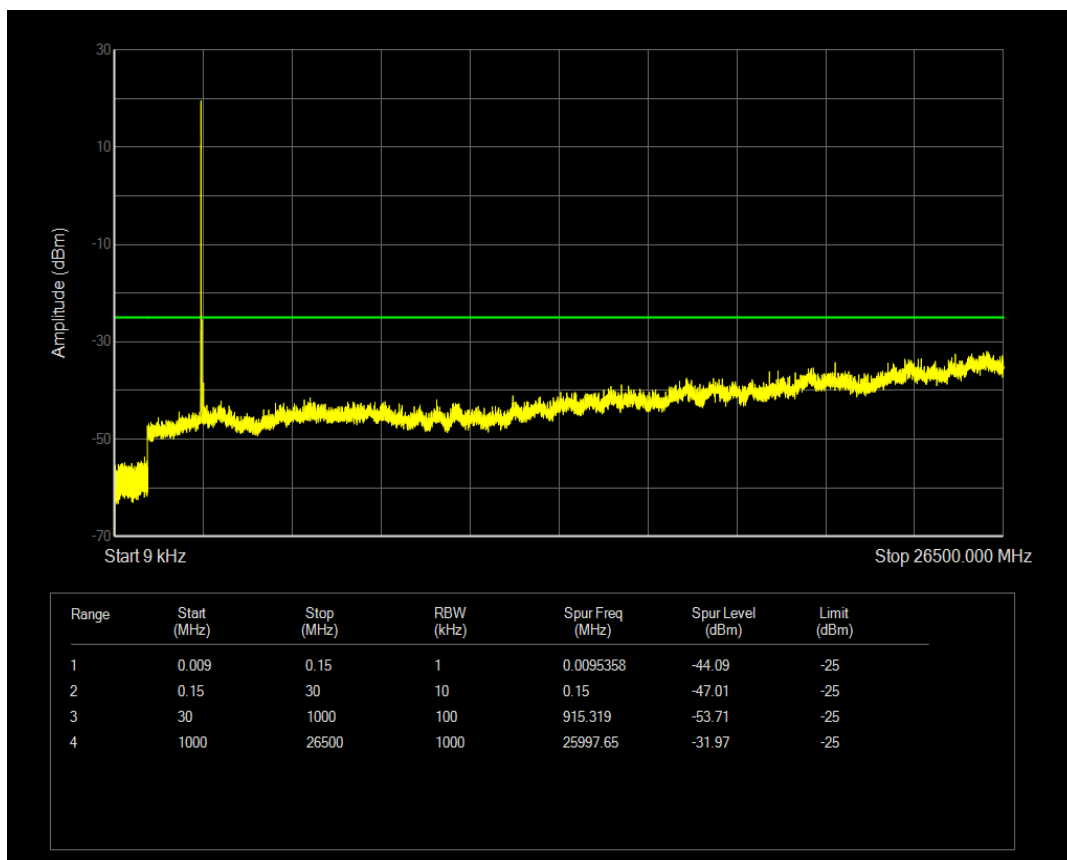
Band41a QPSK BW=5MHz Channel=41215 RB Size=1 Position=#0
