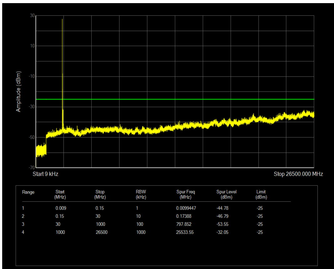
Band41a 16QAM BW=15MHz Channel=40115 RB Size=1 Position=#0
