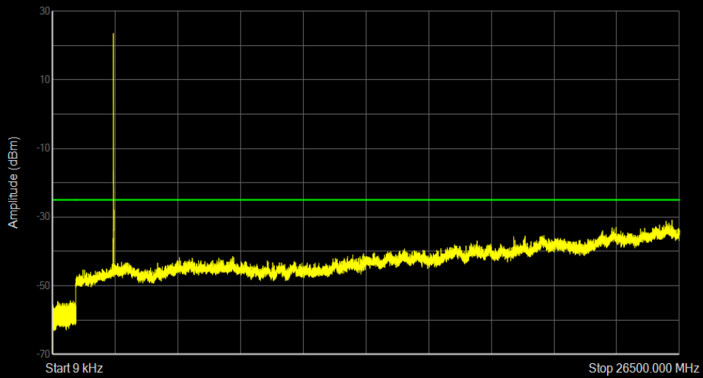
Band41a 16QAM BW=10MHz Channel=40640 RB Size=1 Position=#0
