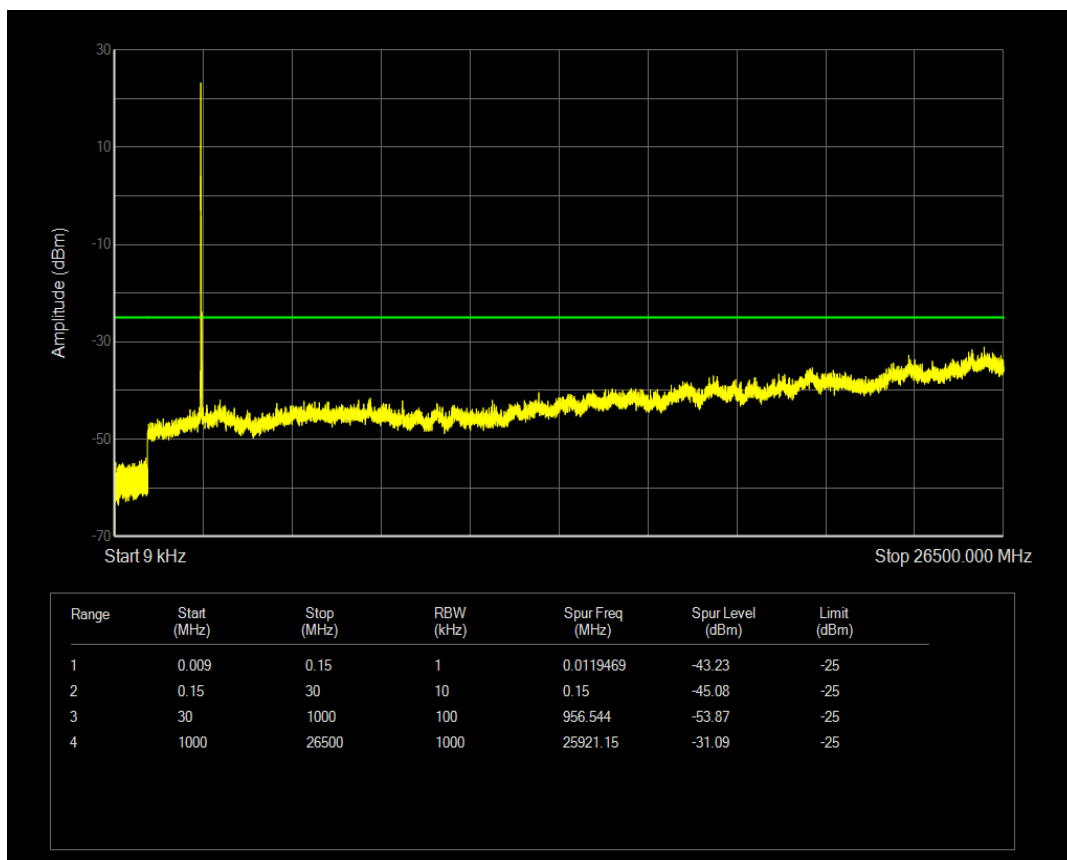
Band41a QPSK BW=15MHz Channel=40640 RB Size=75 Position=#0
