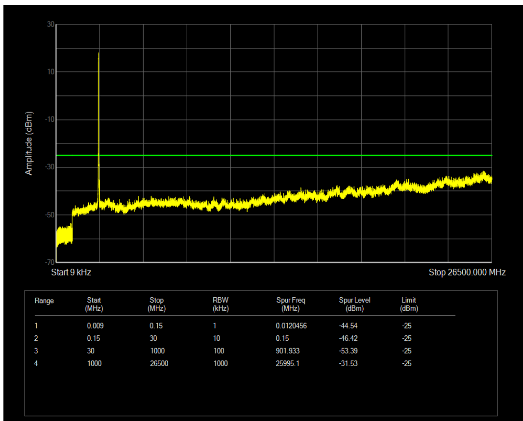
Band41a 16QAM BW=20MHz Channel=40640 RB Size=1 Position=#0
