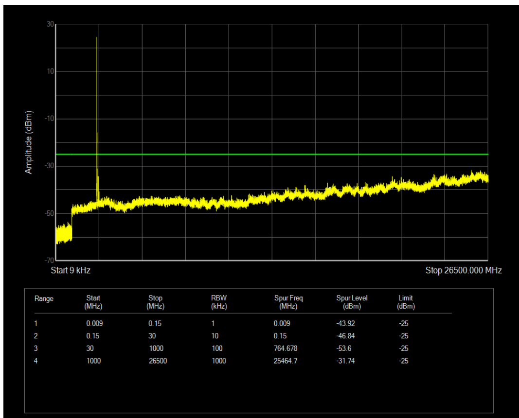
Band41a 16QAM BW=10MHz Channel=40090 RB Size=1 Position=#0
