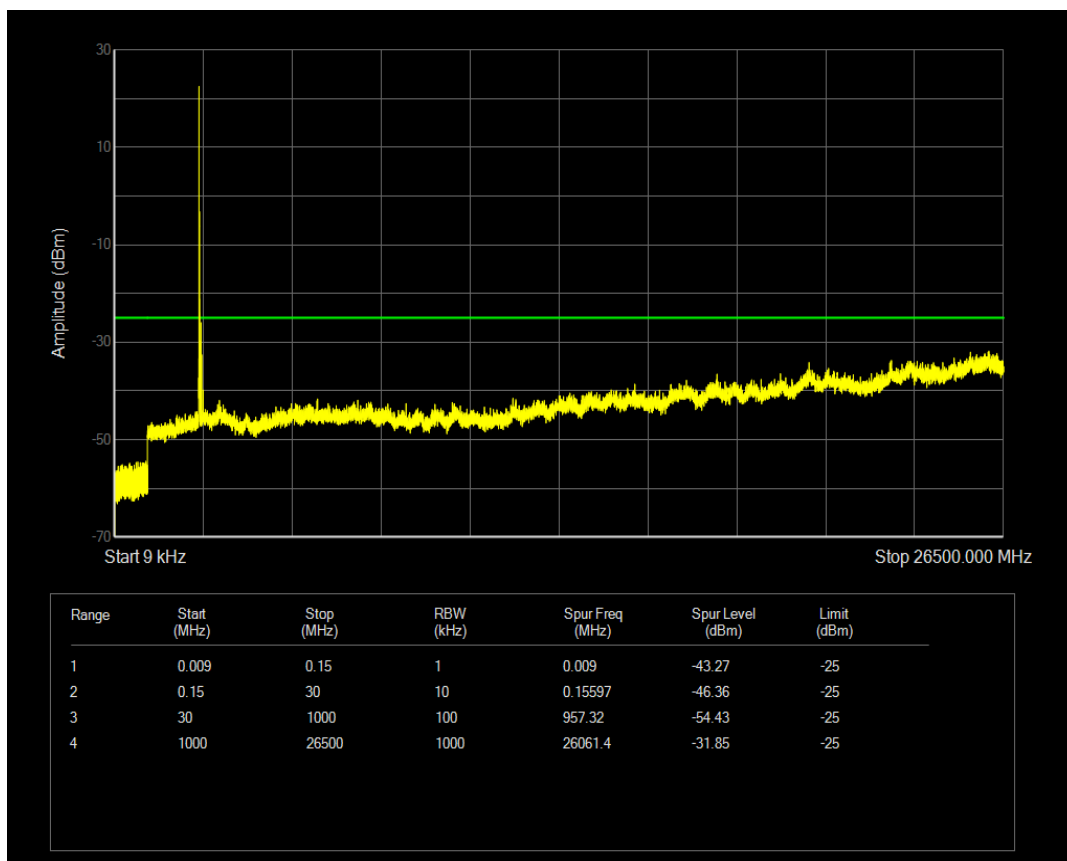
Band41a 16QAM BW=15MHz Channel=40115 RB Size=75 Position=#0
