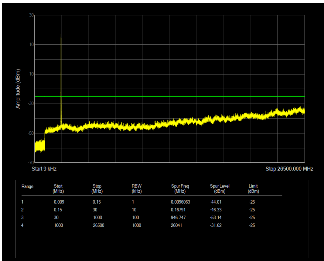
Band41a QPSK BW=15MHz Channel=41165 RB Size=1 Position=#0
