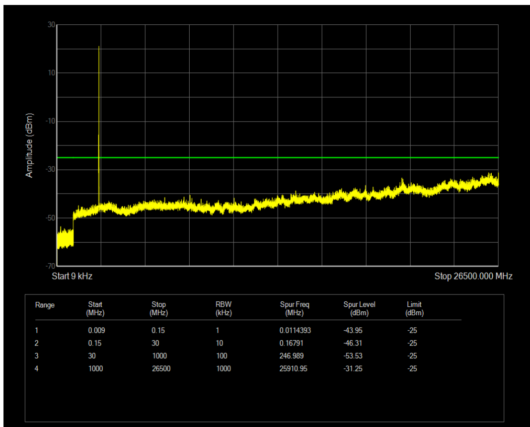
Band41a 16QAM BW=5MHz Channel=40065 RB Size=1 Position=#0
