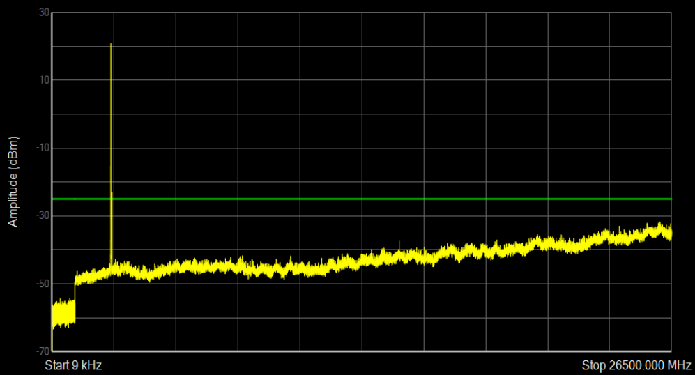
Band41a 16QAM BW=5MHz Channel=40065 RB Size=25 Position=#0
