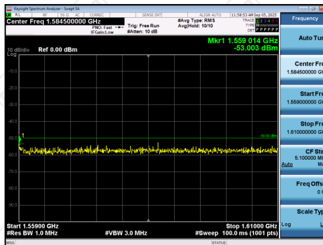
Band13-5MHz-QPSK-23230-1RB#0-Range5:1559~1610MHz
