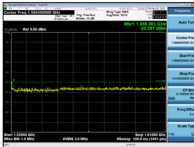
Band13-5MHz-QPSK-23255-1RB#0-Range5:1559~1610MHz
