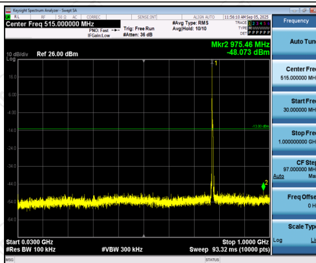
Band13-5MHz-QPSK-23205-1RB#0-Range1:30~1000MHz
