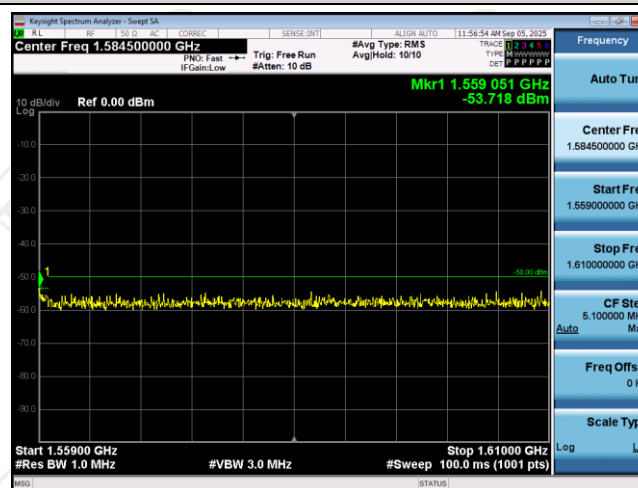
Band13-5MHz-QPSK-23205-1RB#0-Range5:1559~1610MHz
