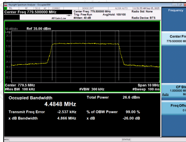
Band13-5MHz-QPSK-23205-25RB#0
