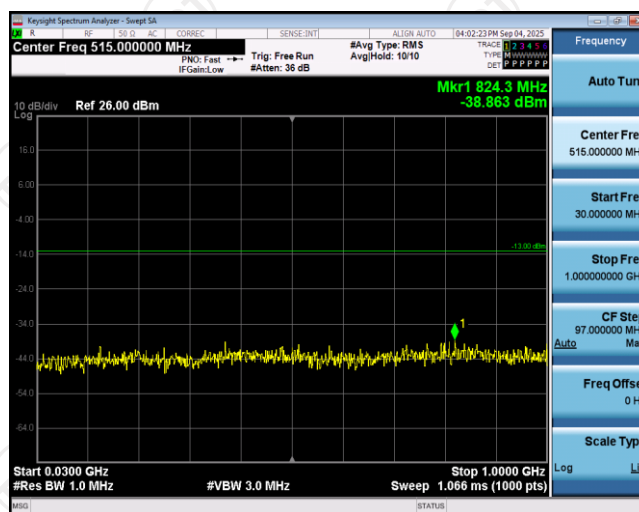
Band2-20MHz-16QAM-19100-1RB#0-Range1:30~1000MHz
