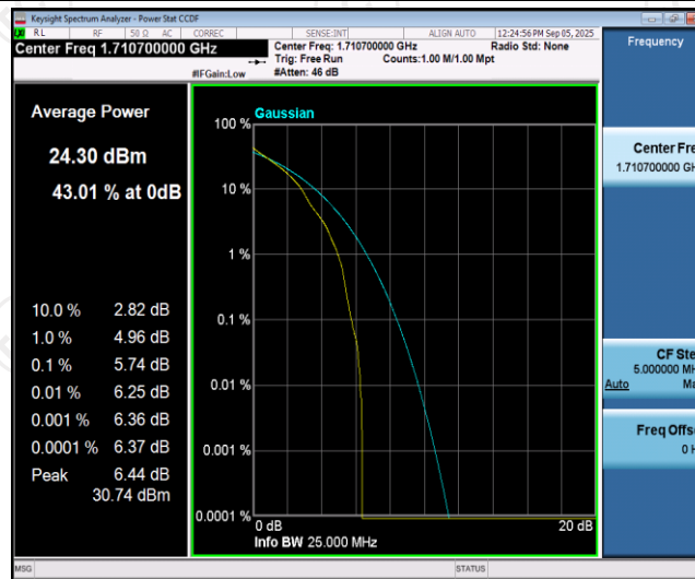
Band66-1.4MHz-QPSK-131979-1RB#0
