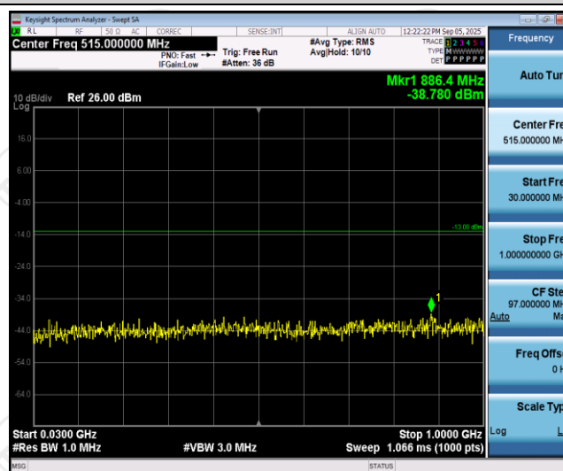
Band66-1.4MHz-16QAM-131979-1RB#0-Range1:30~1000MHz
