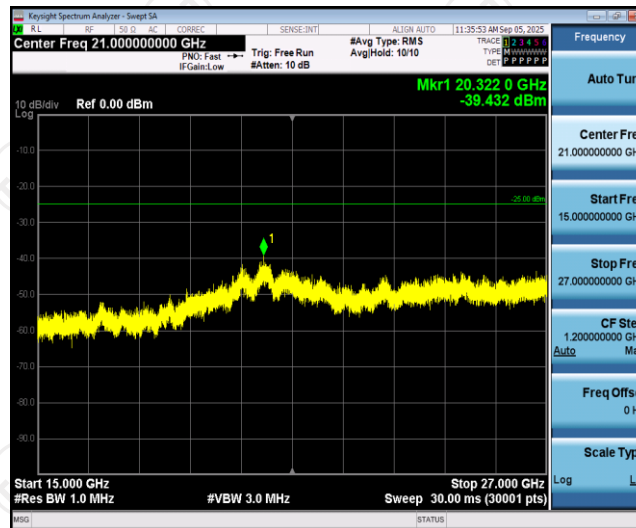
Band7-15MHz-16QAM-20825-1RB#0-Range3:15000~27000MHz
