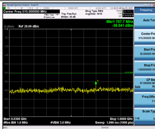
Band7-15MHz-16QAM-21100-1RB#0-Range1:30~1000MHz
