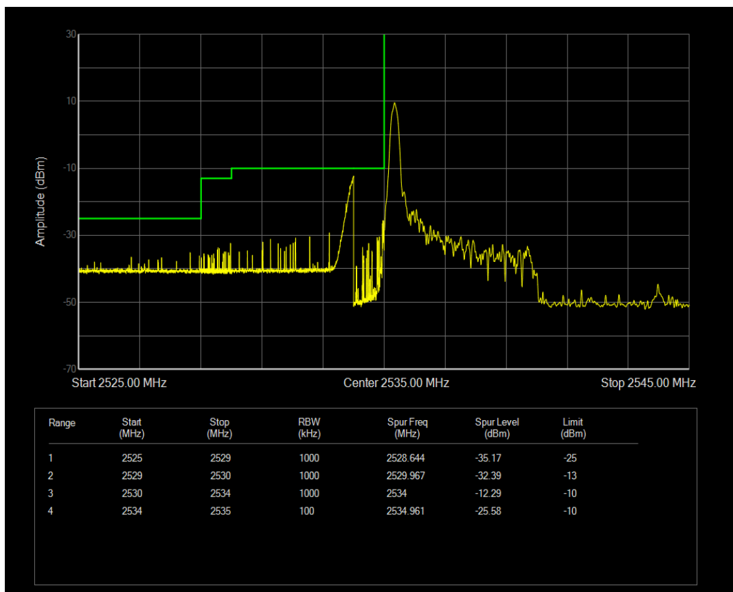
Band41(2535-2655) 16QAM BW=5MHz Channel=40065 RB Size=1 Position=#Max
