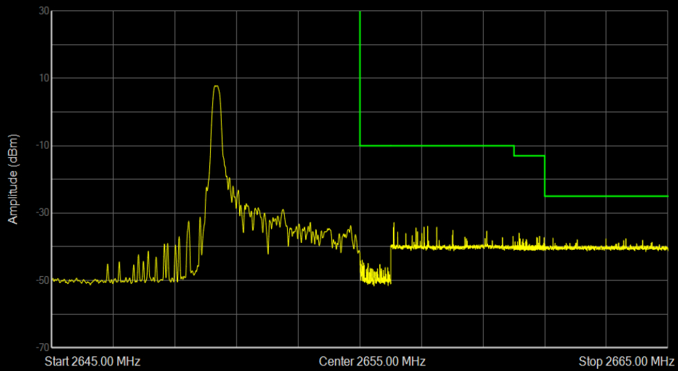
Band41(2535-2655) QPSK BW=5MHz Channel=41215 RB Size=1 Position=#0
