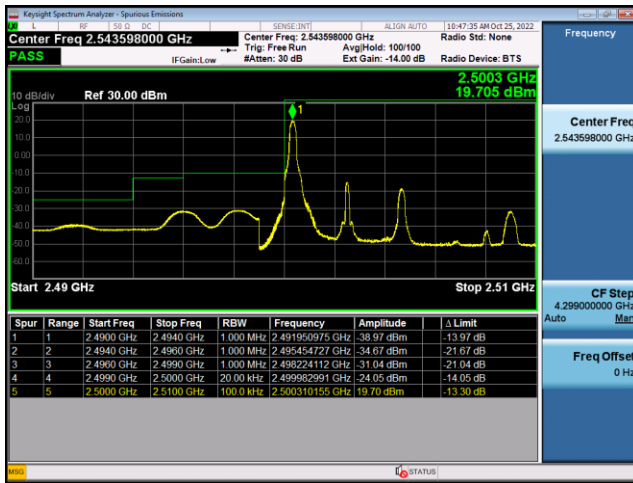
FDD7-5MHz-QPSK-LCH-25RB#0
