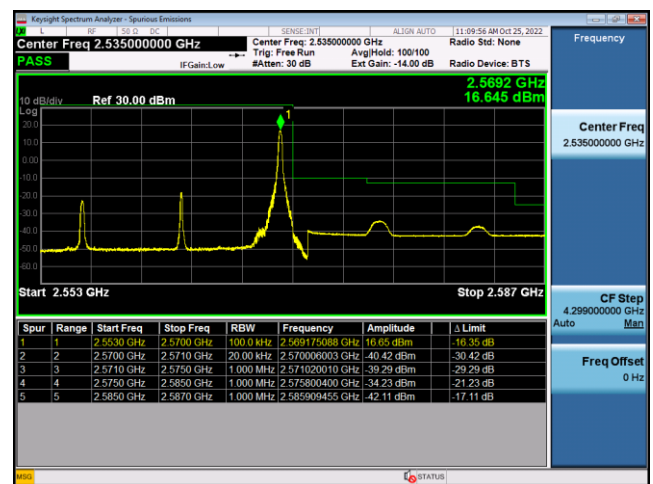
FDD7-15MHz-16QAM-HCH-75RB#0
