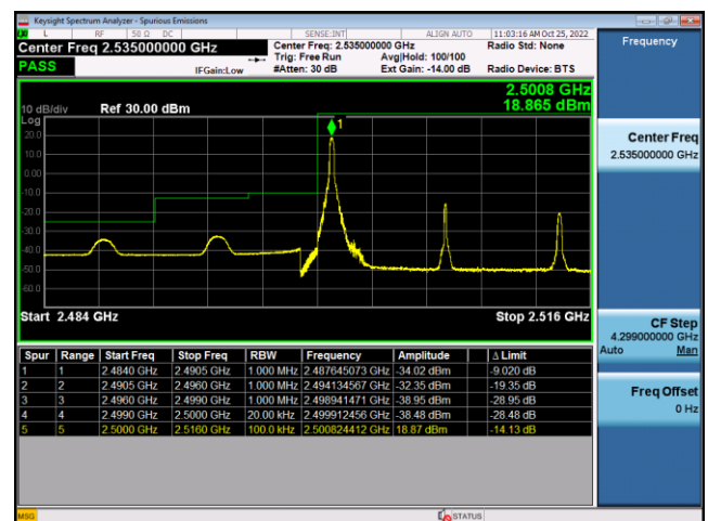
FDD7-15MHz-16QAM-LCH-1RB#0
