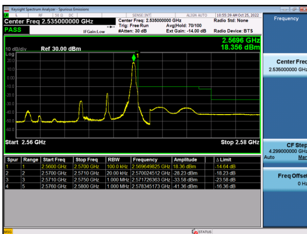
FDD7-5MHz-QPSK-HCH-1RB#24
