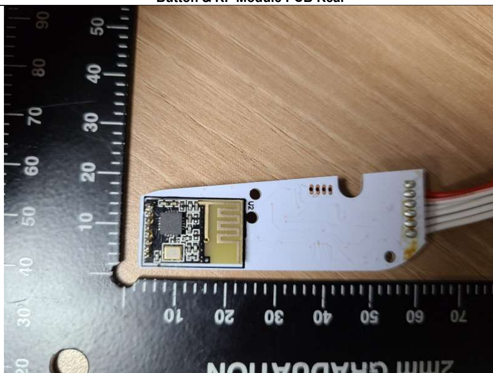
Button & RF Module PCB Rear
