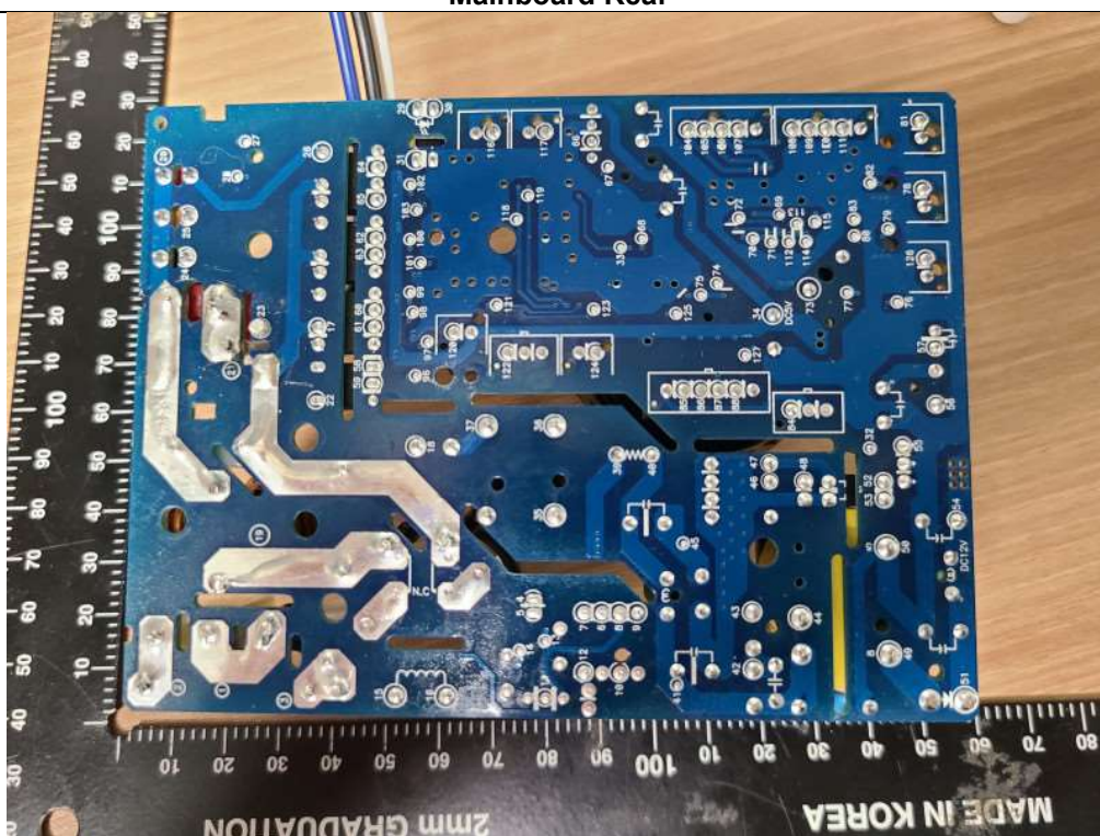
Mainboard Rear
