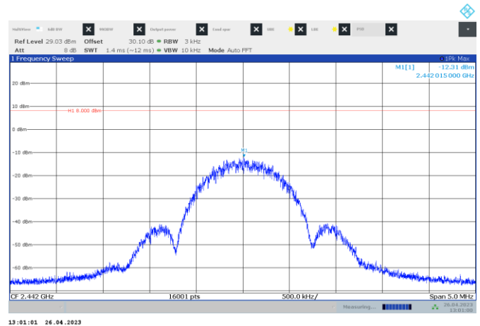
Figure 7.8-2: PSD on mid channel
