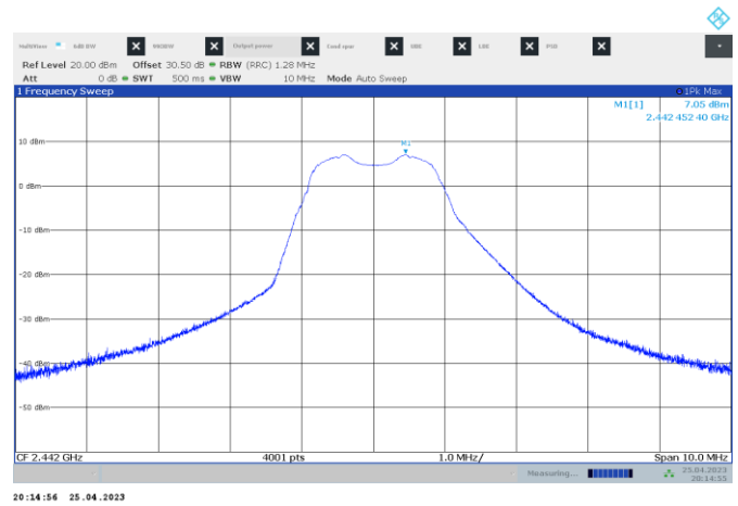
Figure 7.6-2: Output power on mid channel
