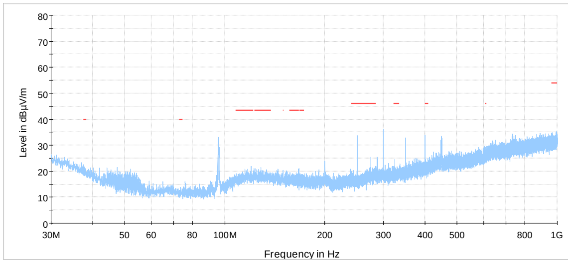
Figure 7.7-4: radiated spurious emissions from 30 MHz to 1000 MHz at low channel
