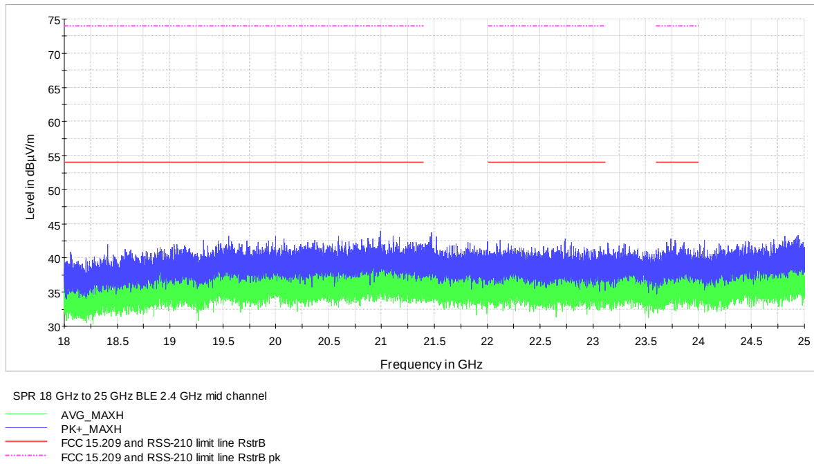
Figure 7.7-10: radiated spurious emissions from 18 GHz to 25 GHz at mid channel
