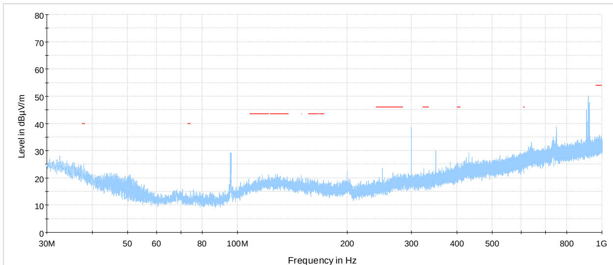
Figure 7.5-10: Radiated spurious emissions from 30 MHz to 1000 MHz at low channel (UNII-2a)
