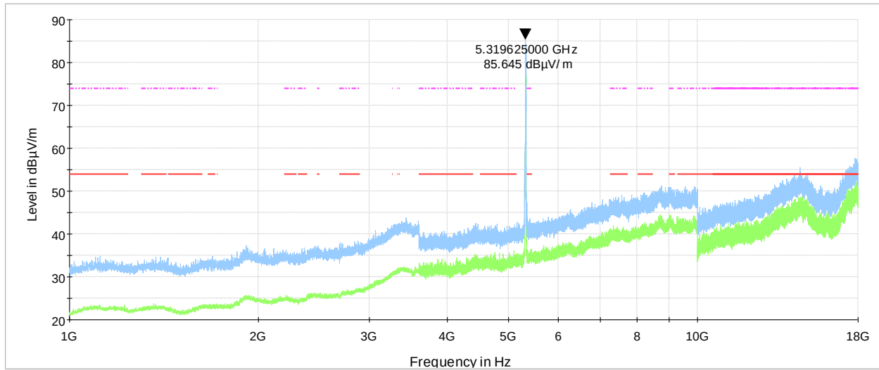
Figure 7.5-14: radiated spurious emissions from 1 GHz to 18 GHz at mid channel (UNII-2a)
