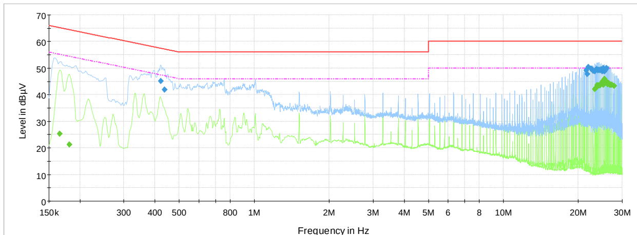
Plot 7.3-1: Conducted emissions on phase line
