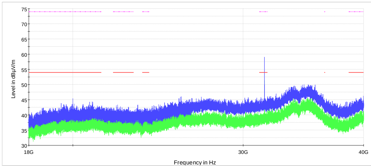
Figure 7.5-7: radiated spurious emissions from 18 GHz to 40 GHz at low channel (UNII-1)
