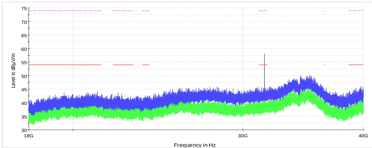
Figure 7.5-16: radiated spurious emissions from 18 GHz to 40 GHz at low channel (UNII-2a)
