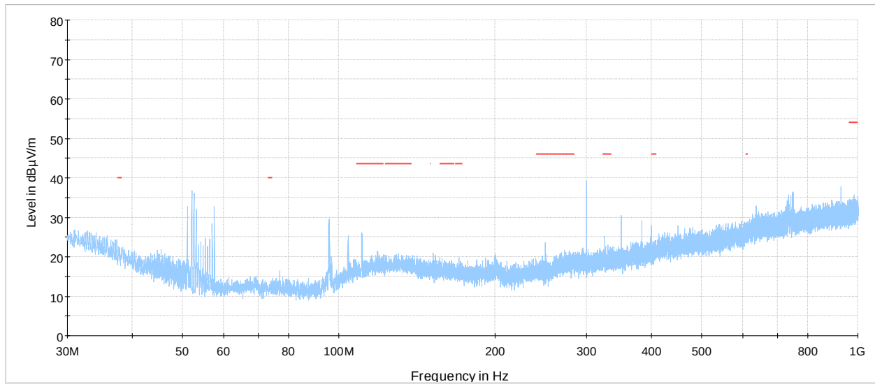
Figure 7.5-1: radiated spurious emissions from 30 MHz to 1000 MHz at low channel (UNII-1)
