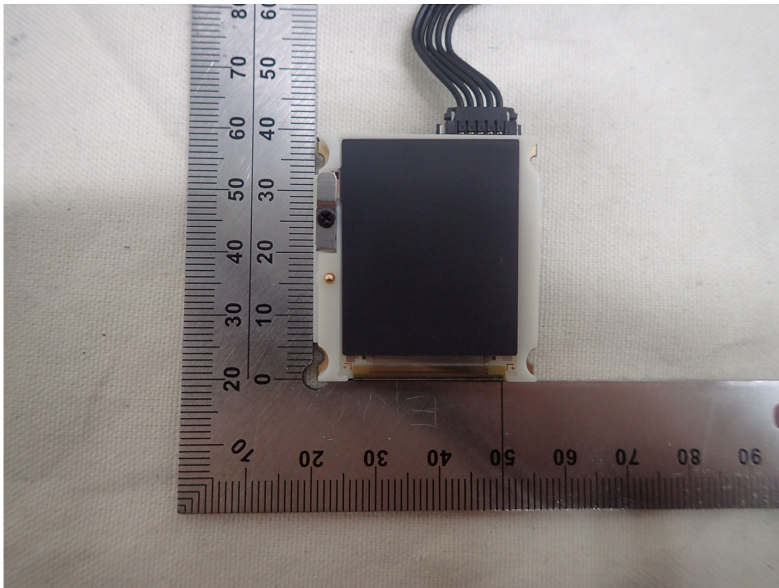
Fingerprint Board Front-1
