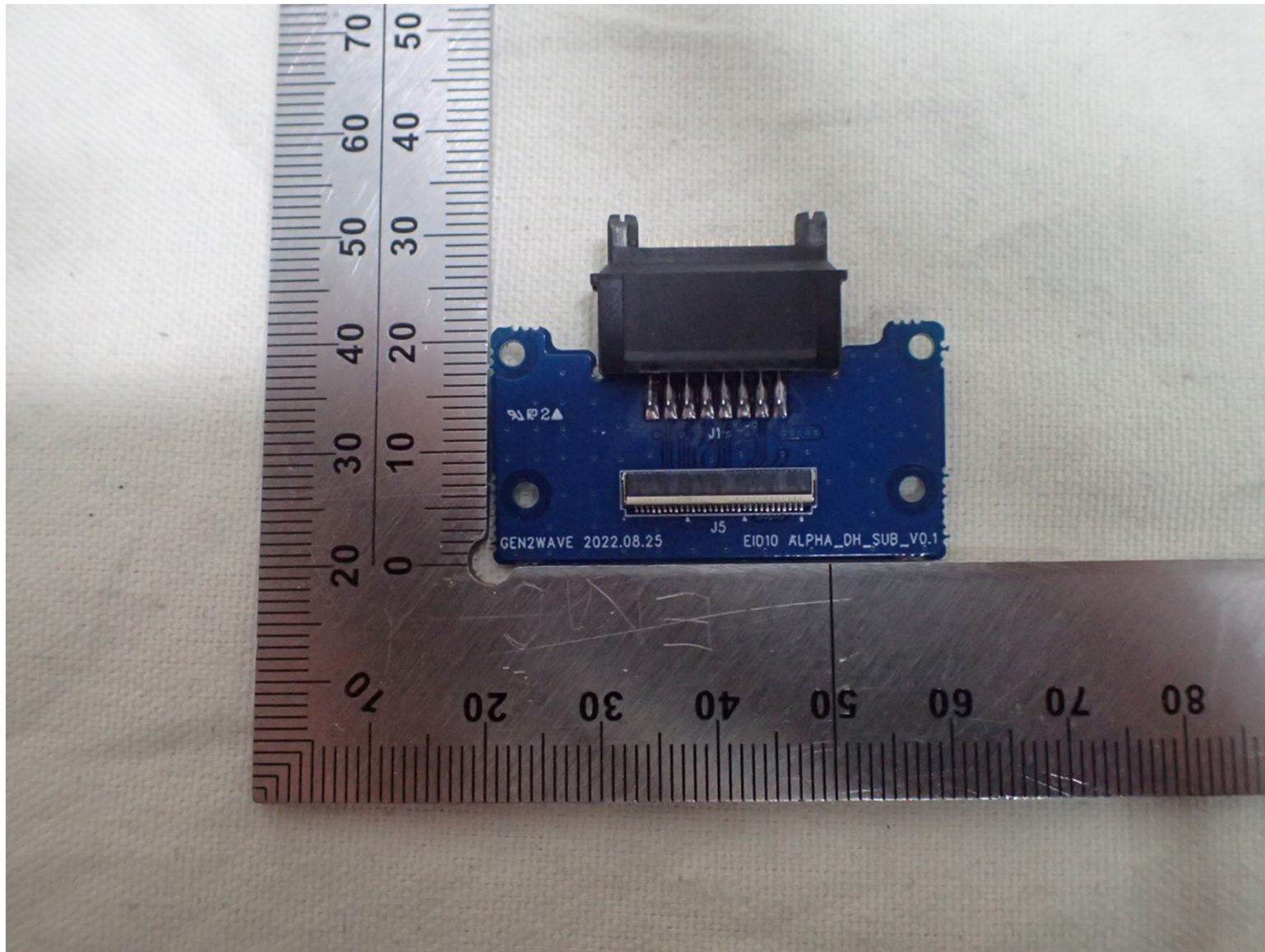
Sub Board Front
