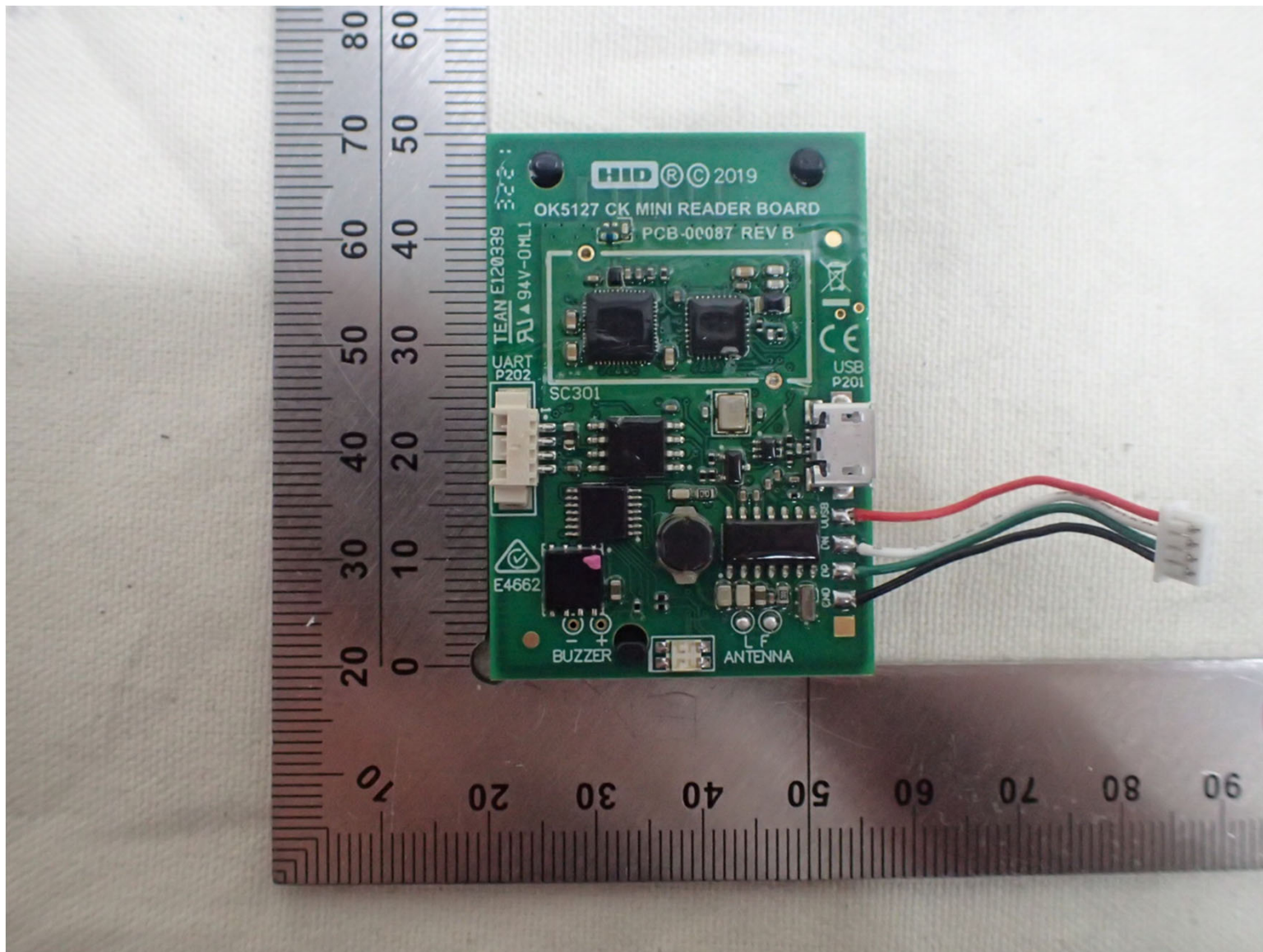
Reader Board Front-2
