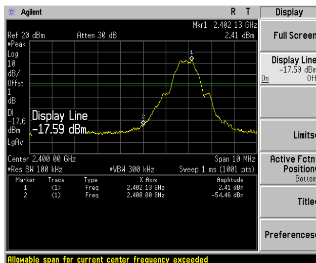
Reference Plot for Channel Frequency 2402MHz
