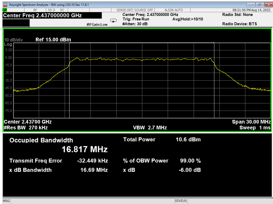
57 6dB Bandwidth, Mid, Wifi G, High Data Rate, conducted
