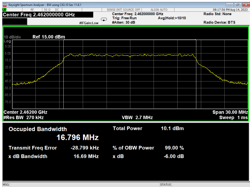
58 6dB Bandwidth, High, Wifi G, High Data Rate, conducted
