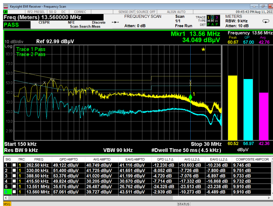
Figure 18 - Conducted Emissions, Neutral, 12% duty cycle, NCEE power supply SN 00077
