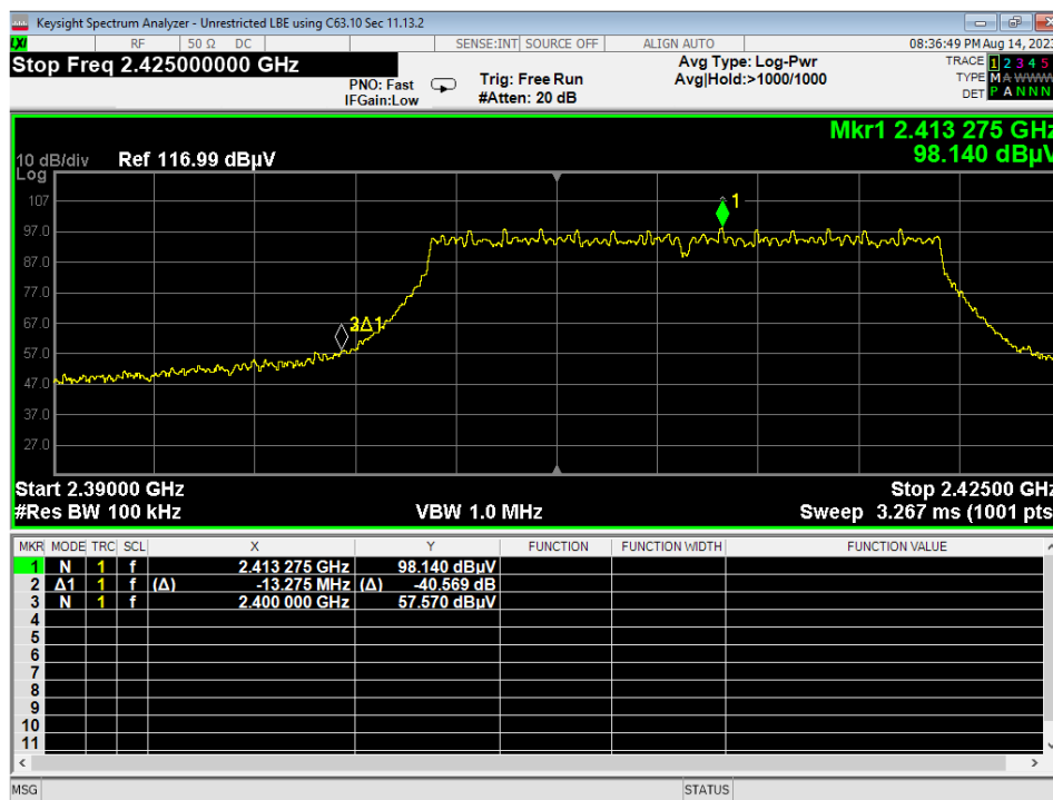
75 Lower Bandedge, Unrestricted, Wifi N, High Data Rate, conducted
