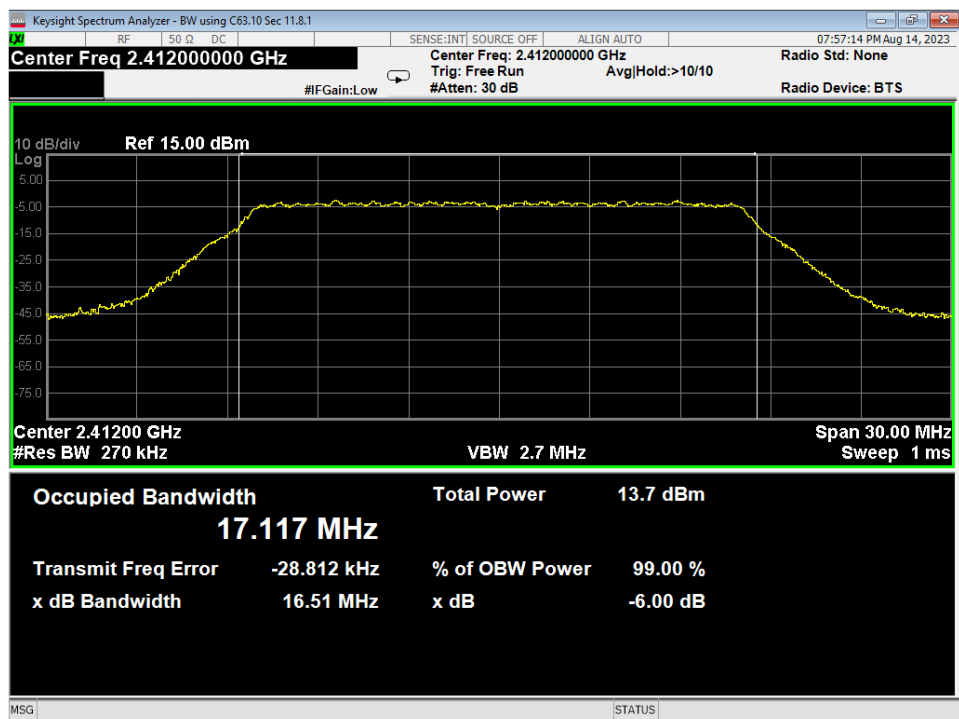
17 6dB Bandwidth, Low, Wifi G, Low Data Rate, conducted
