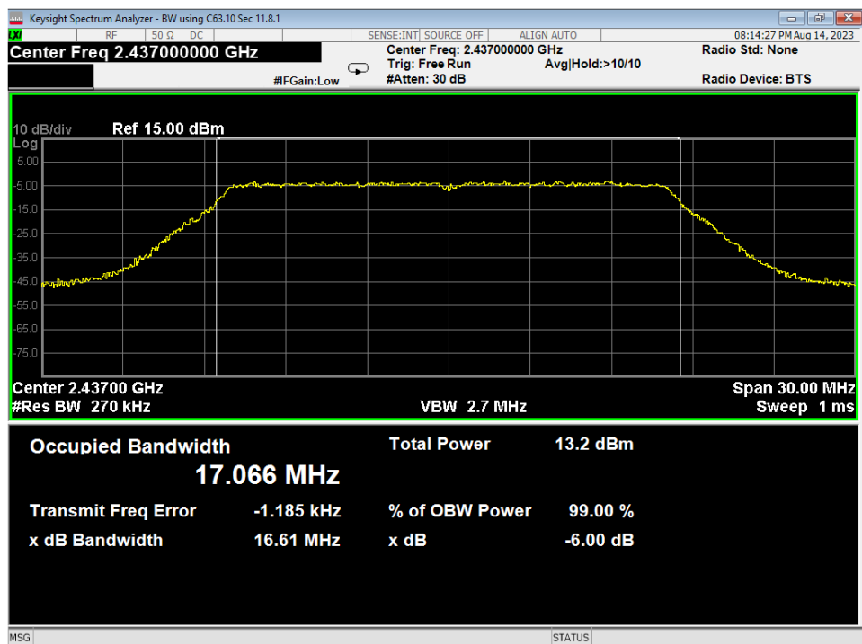
18 6dB Bandwidth, Mid, Wifi G, Low Data Rate, conducted
