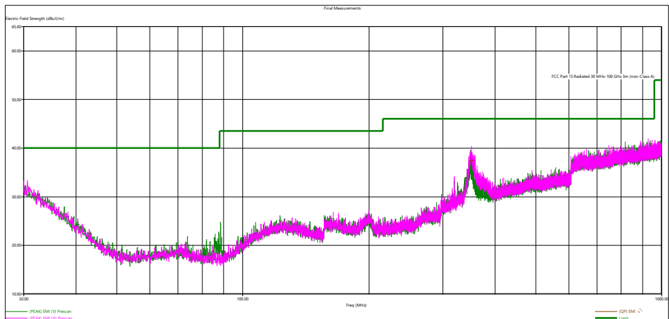
Figure 6 - Radiated Emissions Plot, 802.11g 6MB
