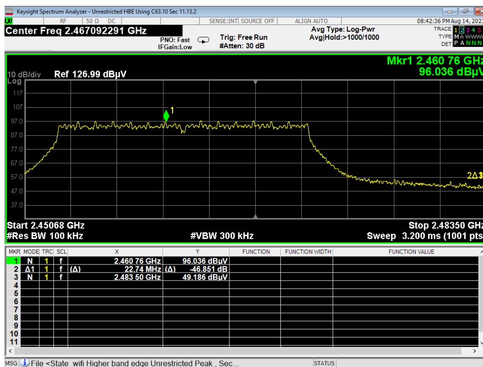
76 Higher Bandedge, Unrestricted, Wifi N, High Data Rate, conducted
