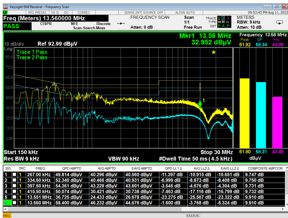
Figure 6 – Conducted Emissions Plot, Line, NFC, 12% RFID duty cycle, SN 00077 power supply
