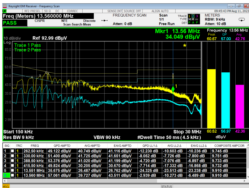
Figure 7 – Conducted Emissions Plot, Neutral, NFC, 12% RFID duty cycle, SN 00077 power supply
