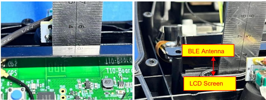
The NRF52811 BLE Antenna to LCD screen Distance (1cm)
