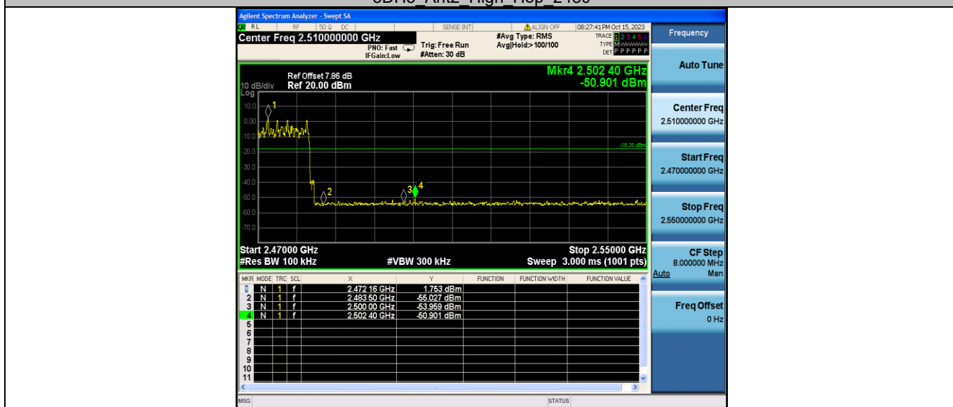
3DH5 Ant2 High Hop 2480
