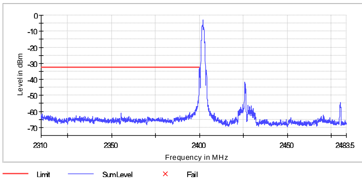
BandEdge
