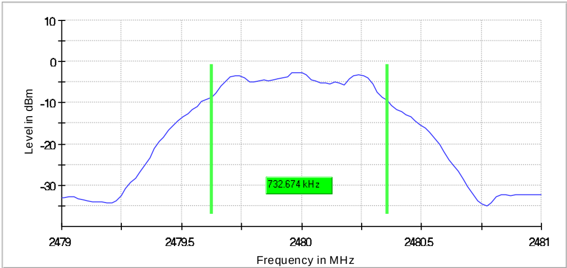
6dBBandwidth
