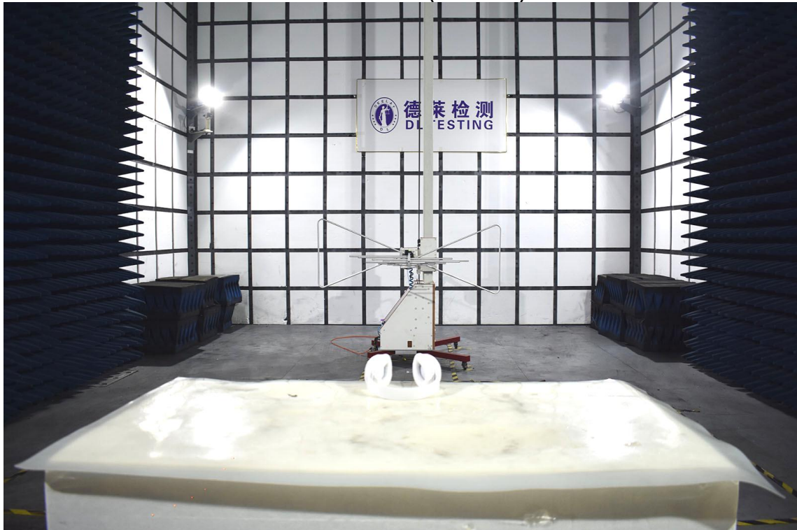
Radiated Emission (Below 1G)
