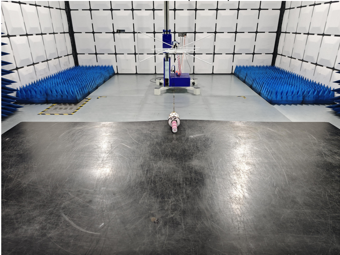
Radiated Emission (Below 1G)
