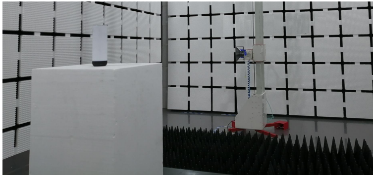
Radiated emission above 1GHz
