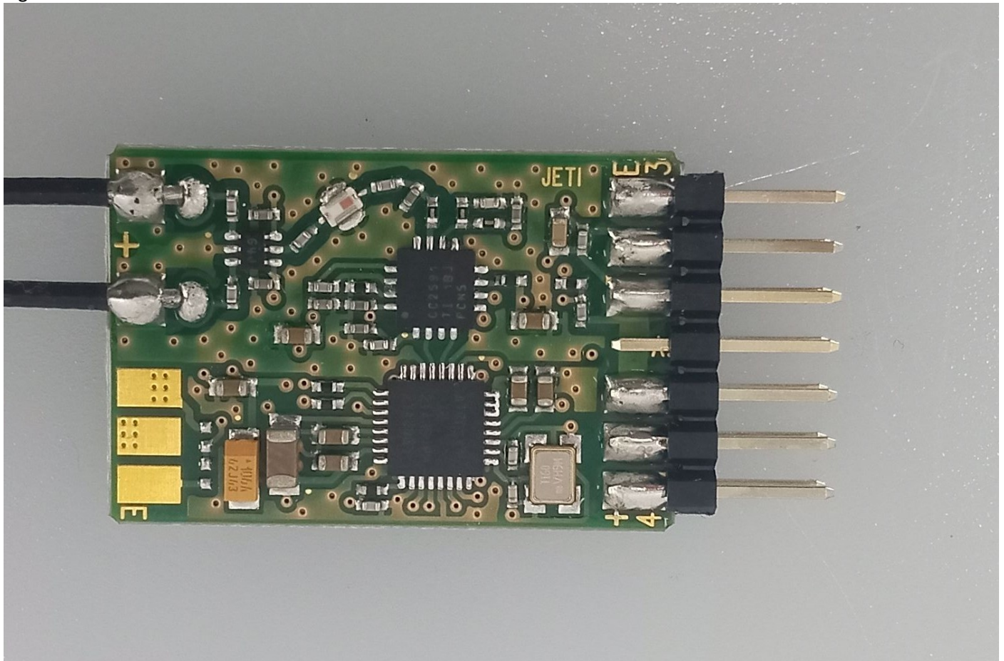
Figure 1 - Front view
