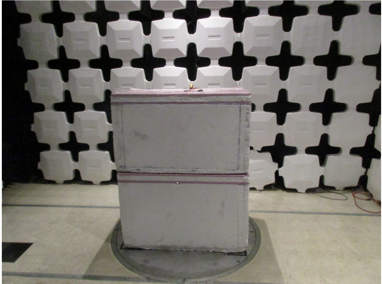
Radiated Testing, Table Setup #2
