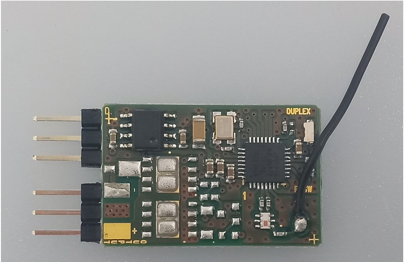
Figure 1 - Front view
