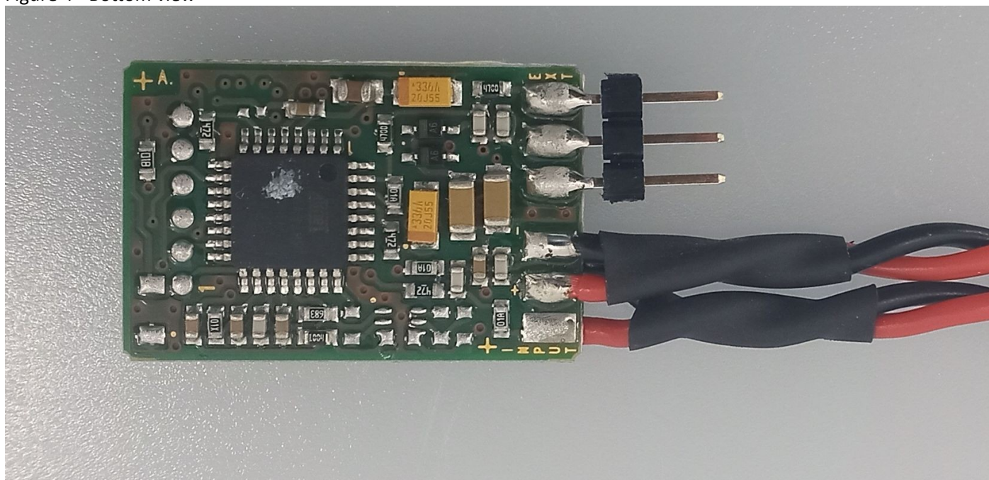
Figure 4 - Bottom view
