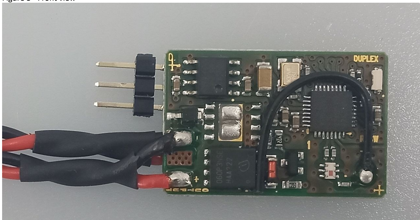
Figure 3 - Front view
