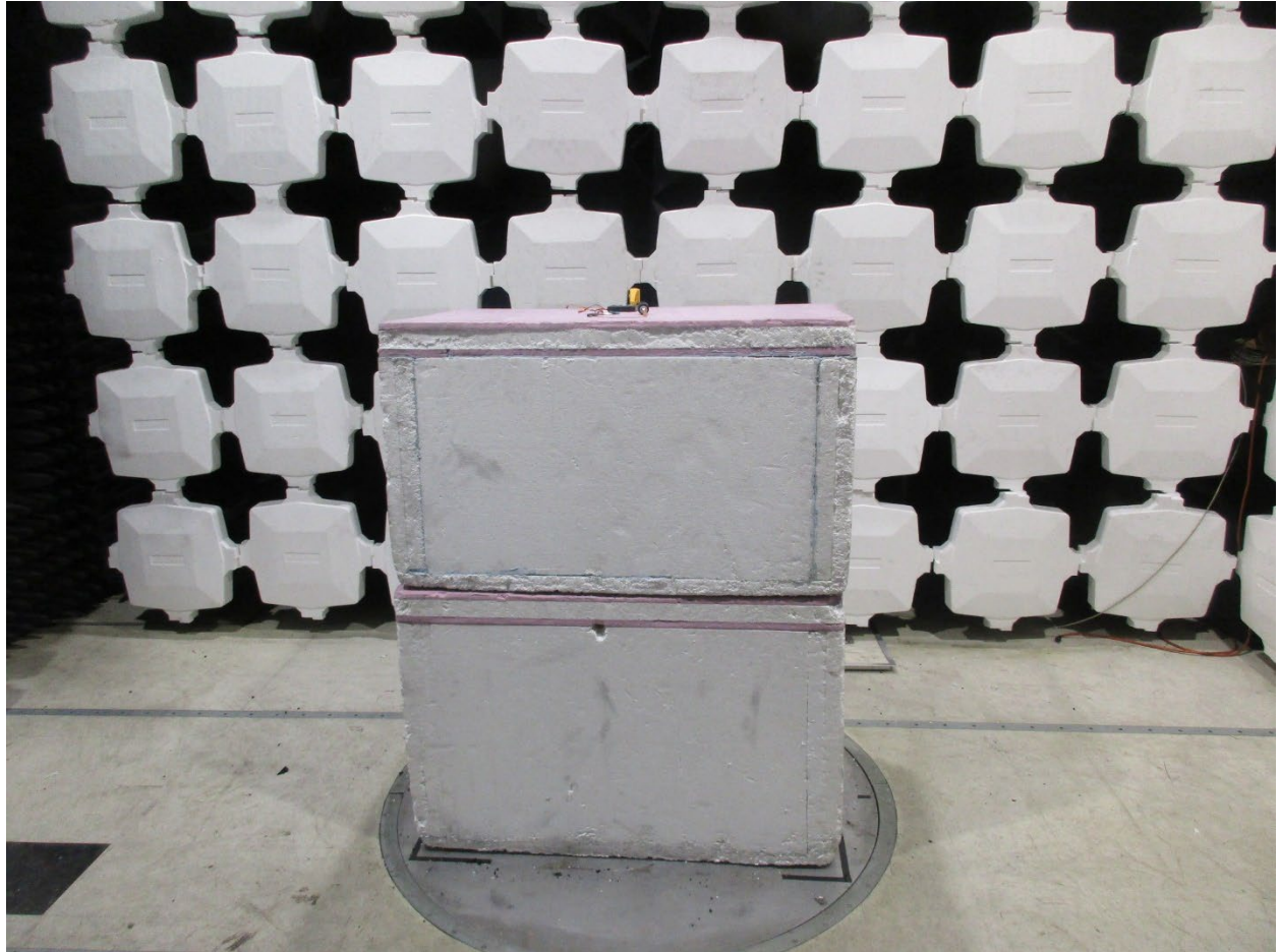
Radiated Testing, Table Setup #2 (15.247)
