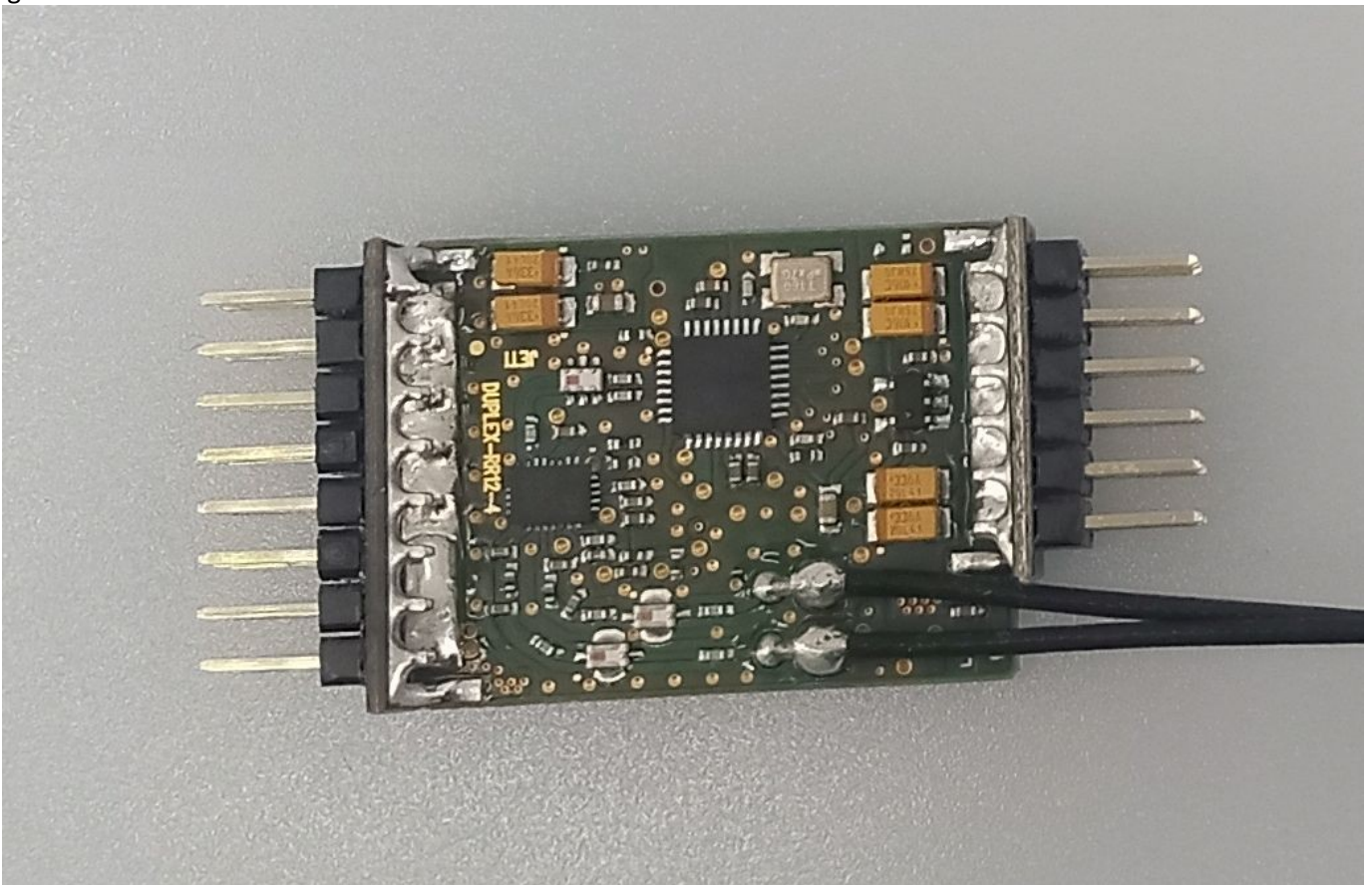
Figure 2 - Bottom view
