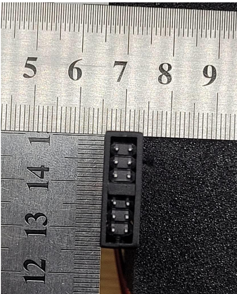
Figure 6 - Bottom view
