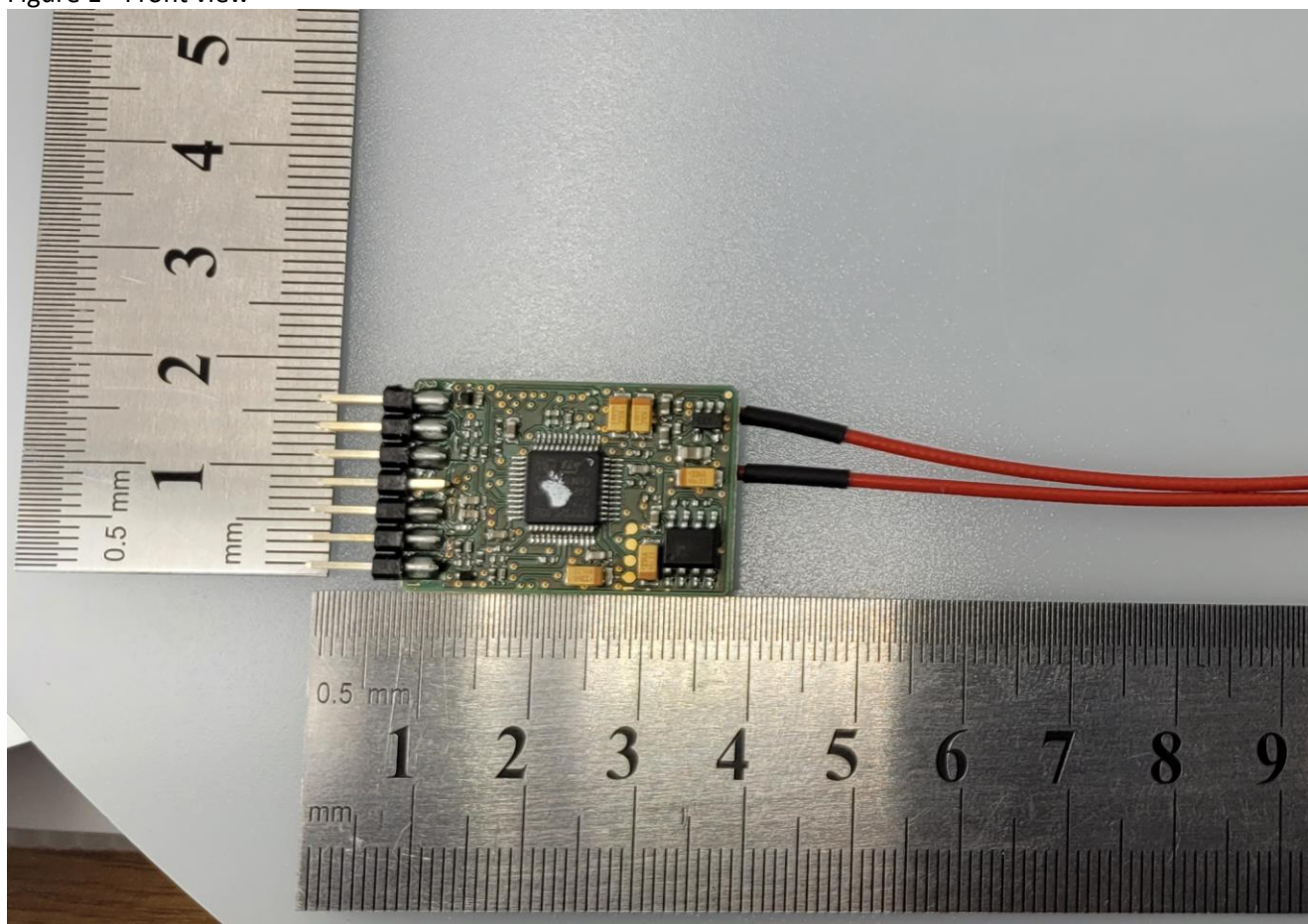
Figure 1 - Front view
