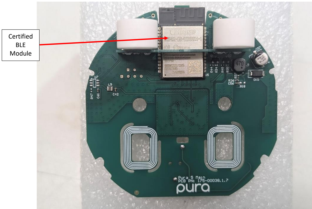
Photograph 1 – Front View of the PCBA
