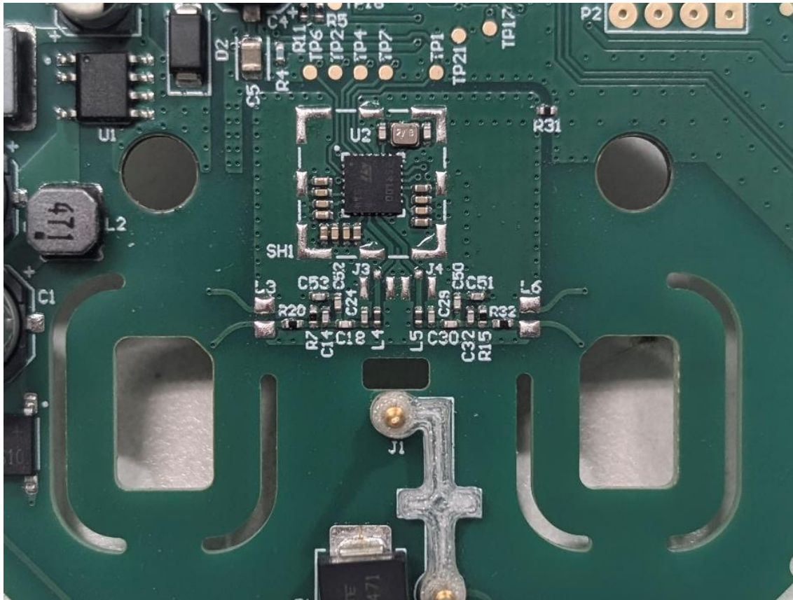
Photograph 3 – Close-up View of the NFC Circuitry
