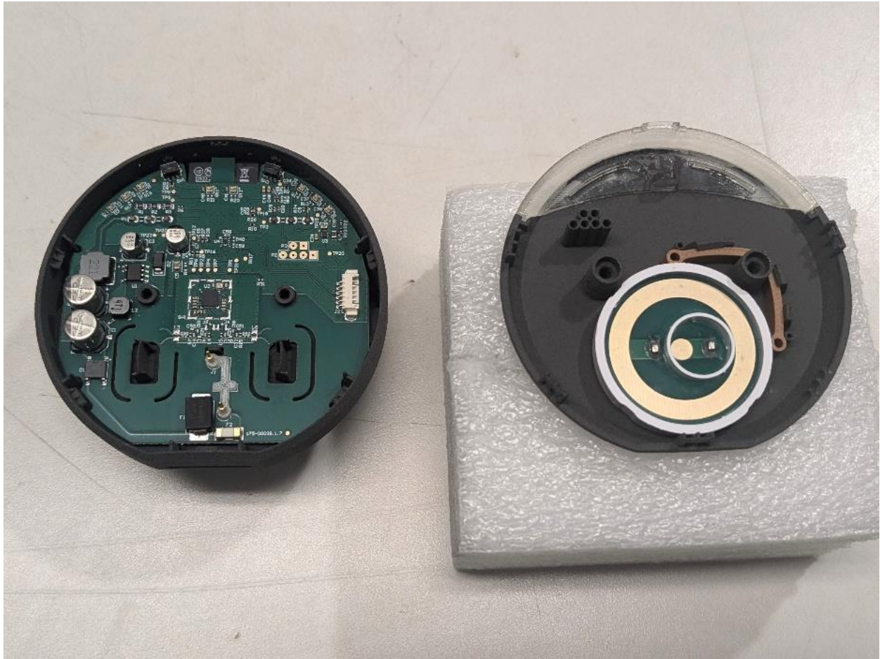
Photograph 4 – View of PCBA in the Housing
