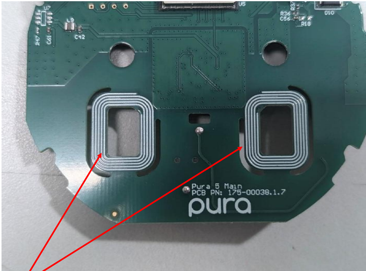
Photograph 5 – View of the NFC Antennas, Back of Board
