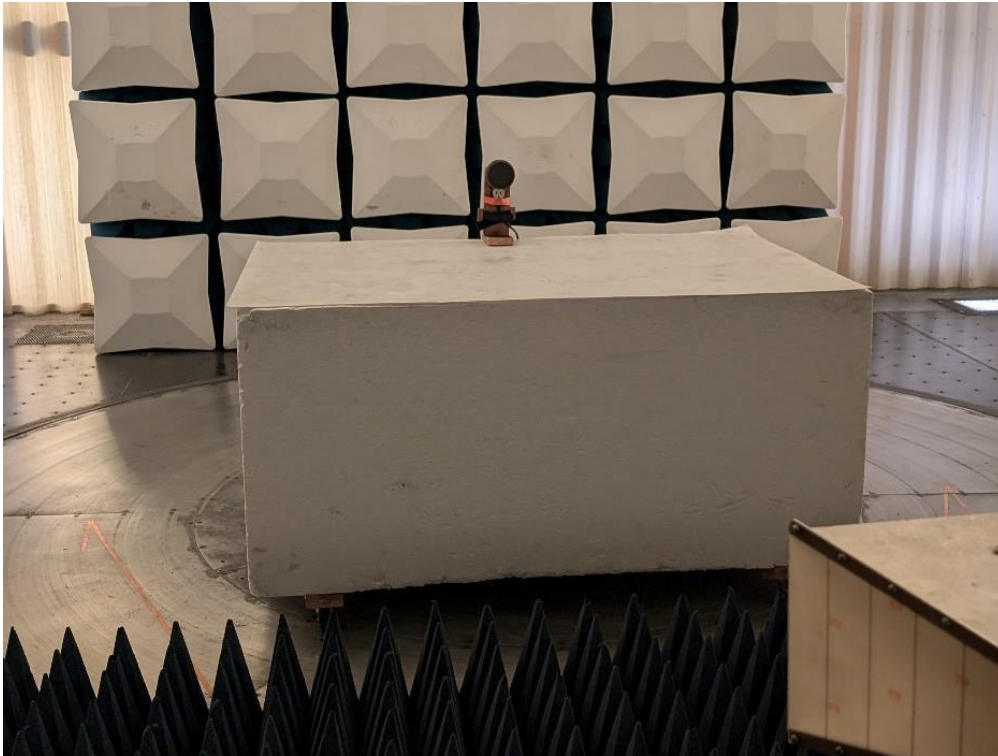
Photograph 5: Front View Radiated Emissions Worst Case – Above 1000MHz Configuration
