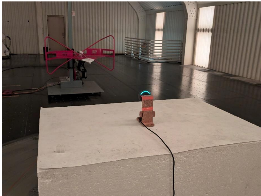
Photograph 2: Back View Radiated Emissions, 30 to 1000 MHz Worst Case Configuration
