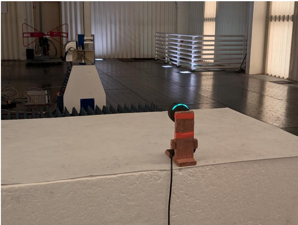
Photograph 6: Back View Radiated Emissions Worst Case – Below 1000 MHz Configuration
