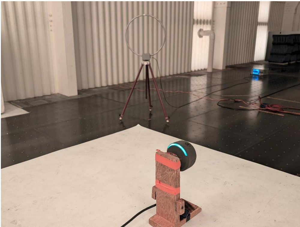
Photograph 4: Back View Radiated Emissions Worst Case – Below 30 MHz Configuration
