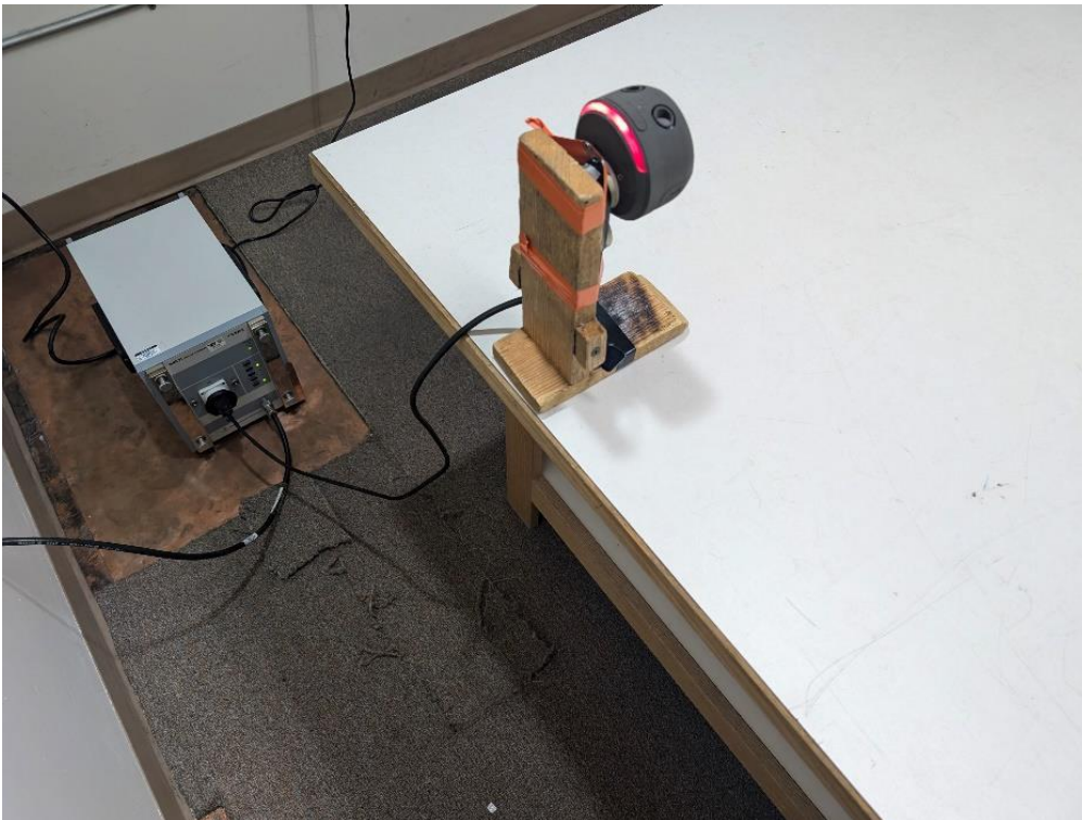
Photograph 8: Back View Conducted Emissions
