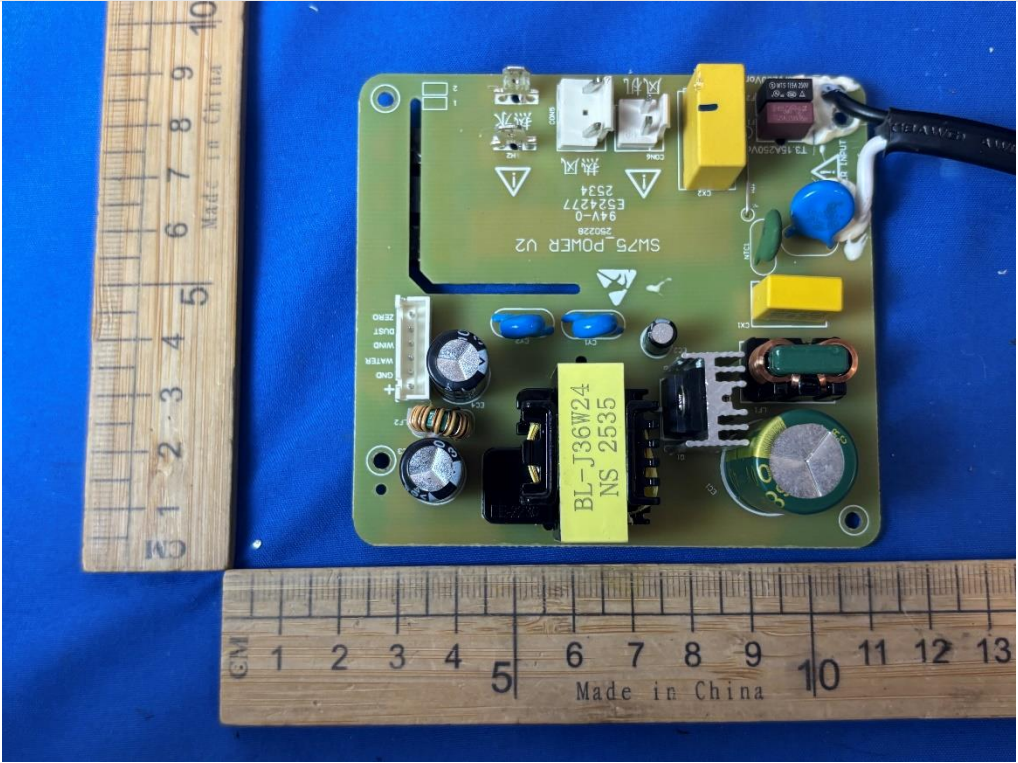
Internal View of EUT-38
