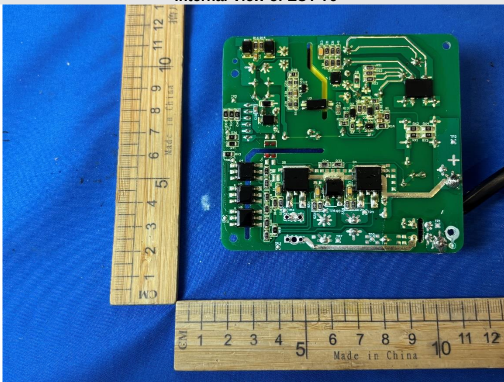
Internal View of EUT-79
