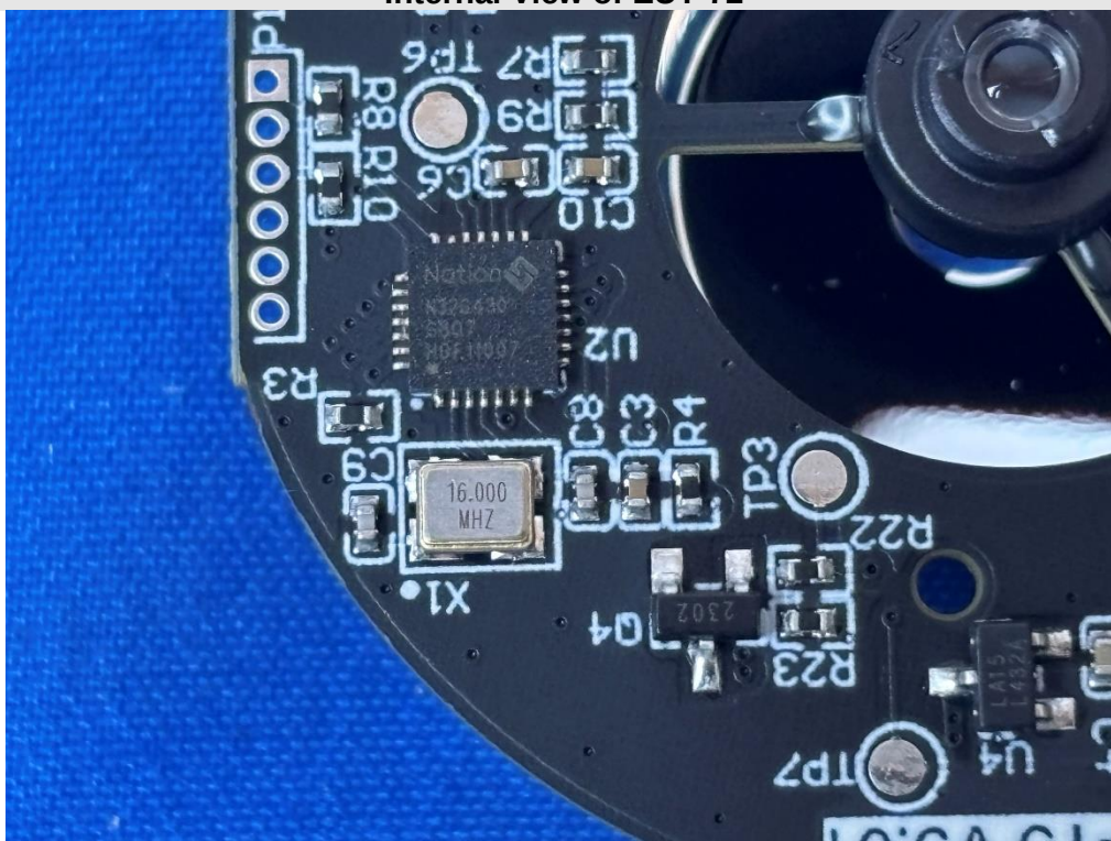
Internal View of EUT-72
