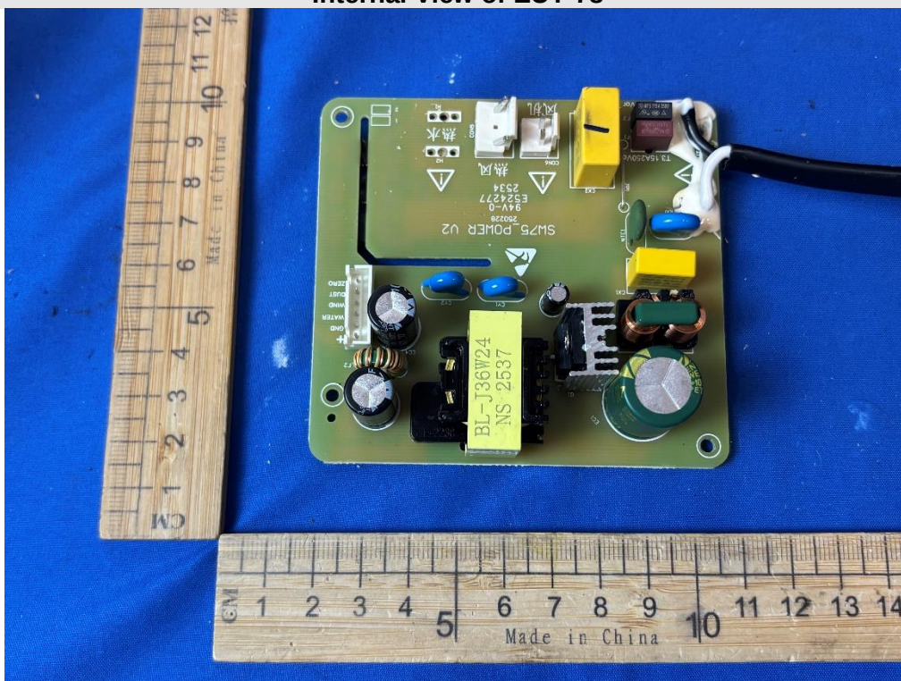
Internal View of EUT-78
