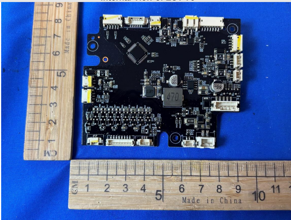
Internal View of EUT-76
