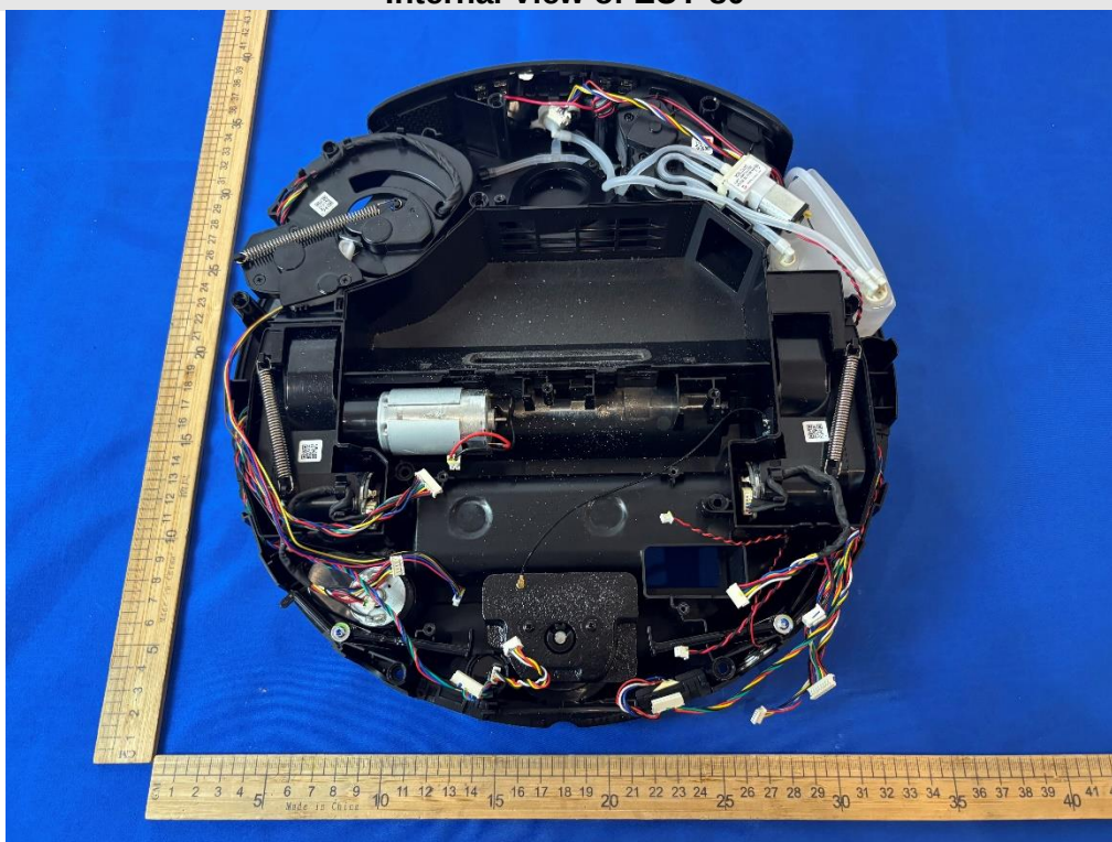
Internal View of EUT-80
