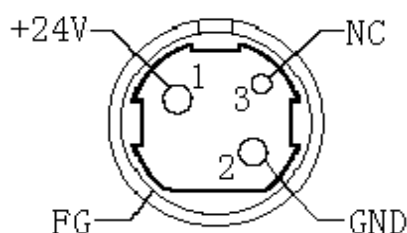
Fig.6.6-2 Schematic drawing of 24V power interface
