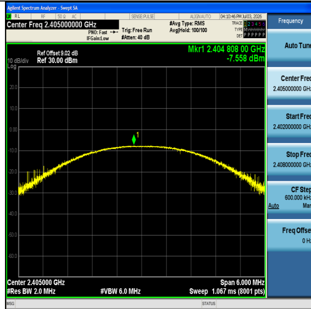
SRD-Ant1-2405-PASS
