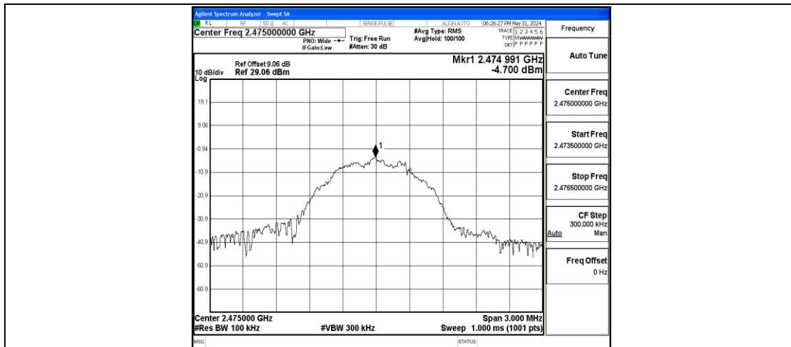
SRD-Ant1-2475-0~Reference-PASS
