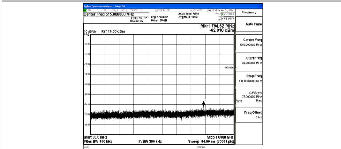
SRD-Ant1-2475-30~1000-PASS
